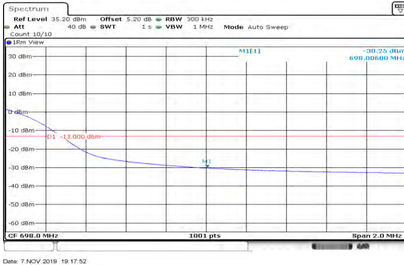
Band71-20MHz-16QAM-133222-1RB#0
