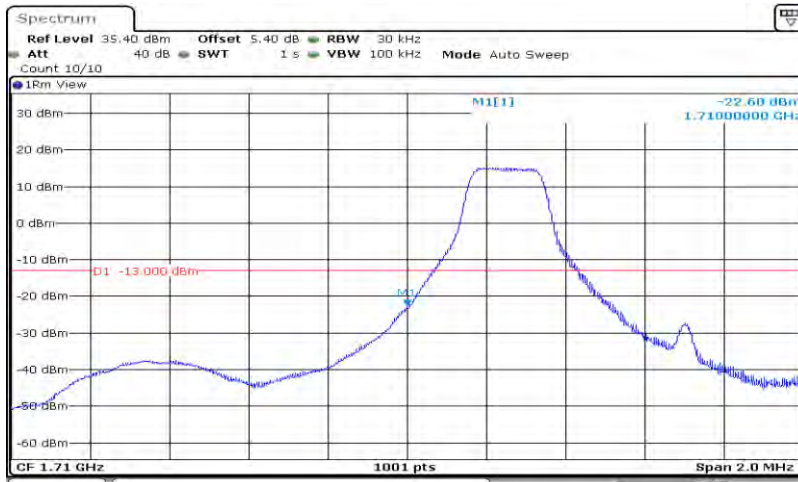
Band66-1.4MHz-16QAM-131979-6RB#0
