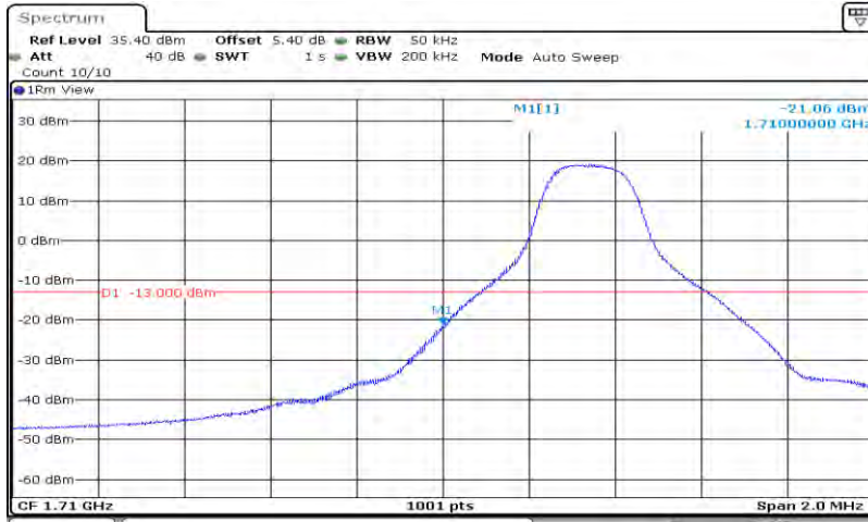
Band66-5MHz-QPSK-131997-25RB#0
