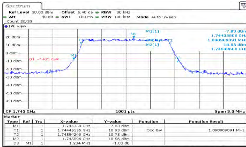
Band66-1.4MHz-QPSK-132322-6RB#0-1.091
