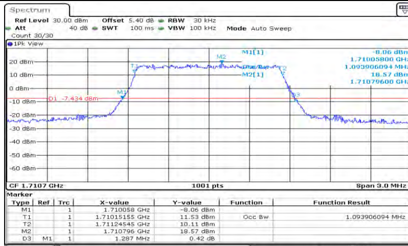
Band66-1.4MHz-QPSK-131979-6RB#0-1.094
