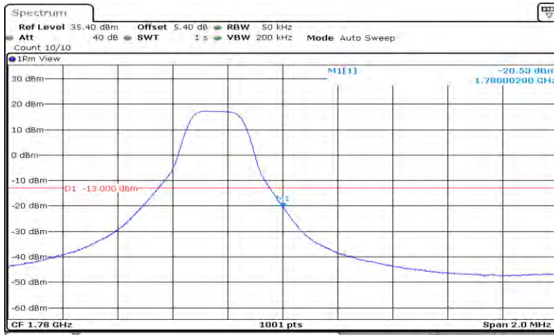
Band66-3MHz-16QAM-132657-15RB#0
