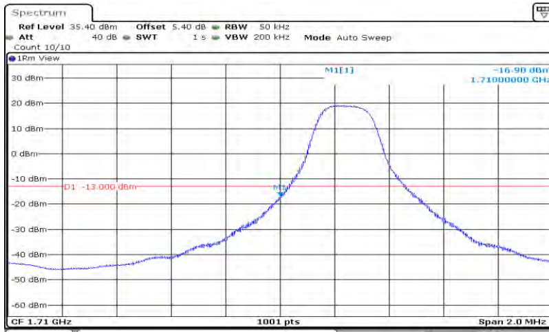
Band66-3MHz-QPSK-131987-15RB#0
