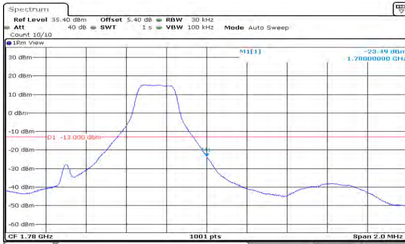
Band66-1.4MHz-16QAM-132665-6RB#0
