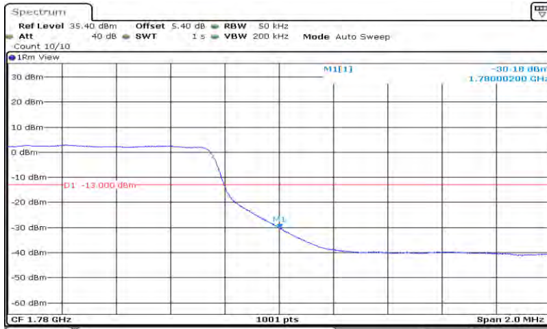
Band66-5MHz-16QAM-132647-25RB#0
