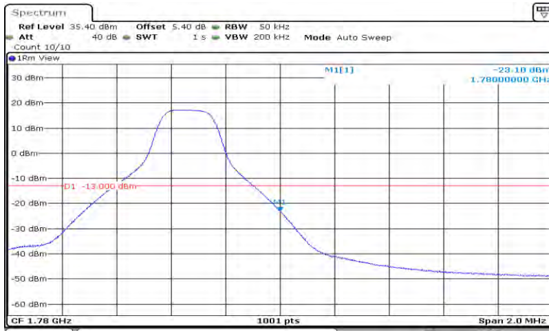
Band66-5MHz-16QAM-132647-25RB#0
