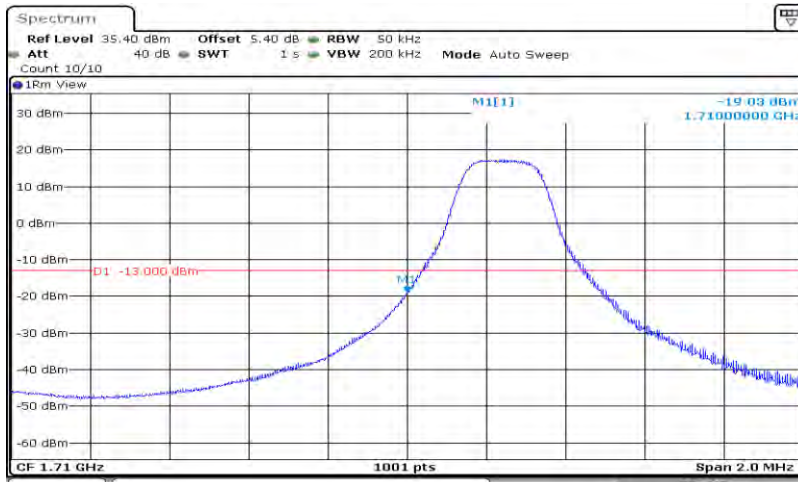
Band66-3MHz-16QAM-131987-15RB#0
