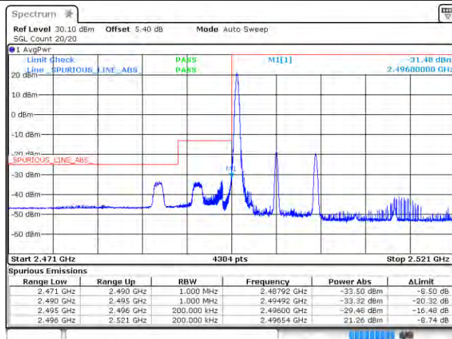
Band41_10MHz_16QAM_39700_50RB#0
