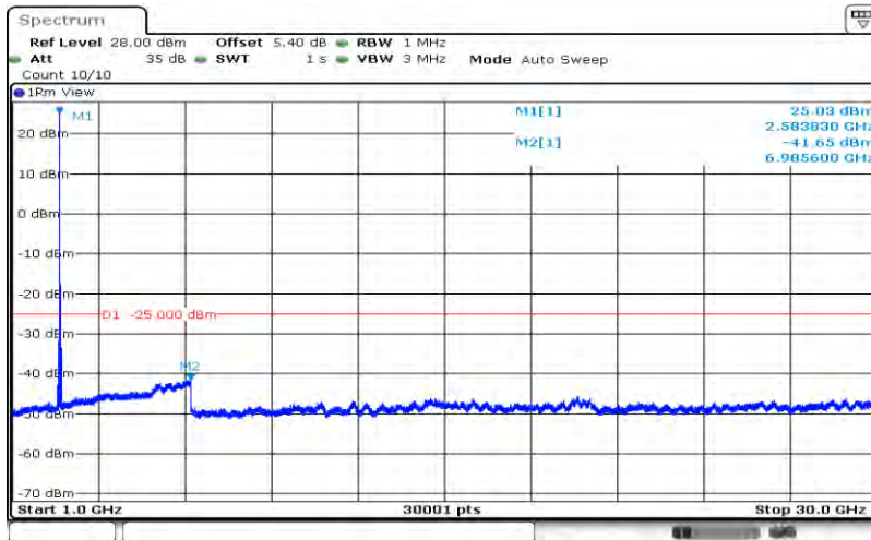
Band41-20MHz-16QAM-40620-1RB#0-Range2:1000~30000MHz
