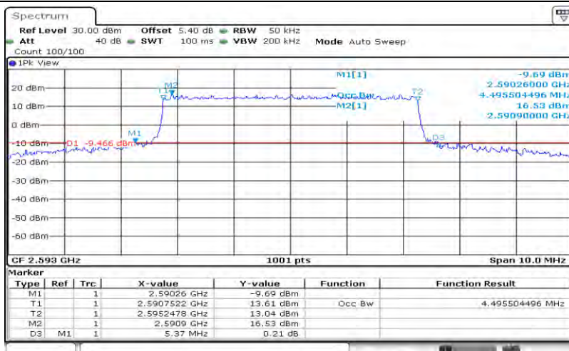
Band41-5MHz-QPSK-40620-25RB#0-4.496
