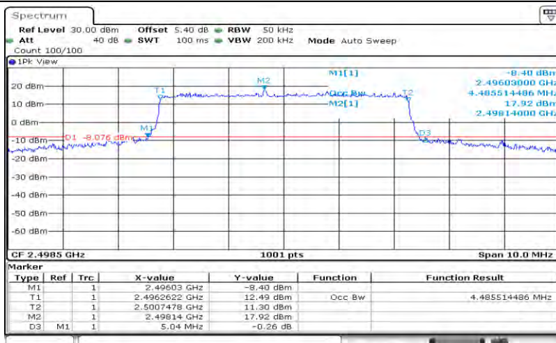
Band41-5MHz-QPSK-39675-25RB#0-4.486
