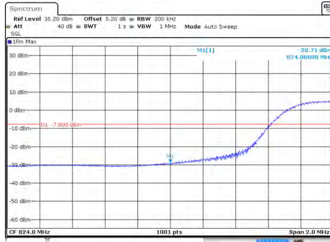
Band 26_15MHz_16QAM_26865_75RB#0
