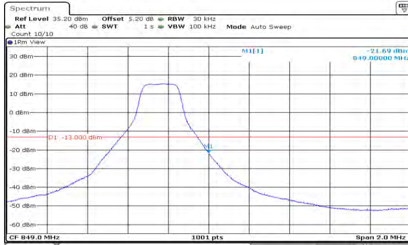
Band 26_3MHz_16QAM_27025_15RB#0
