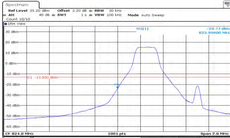
Band 26_1.4MHz_16QAM_26797_6RB#0
