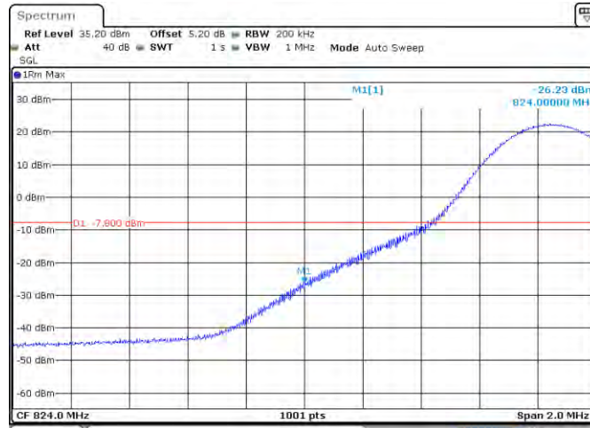
Band 26_15MHz_16QAM_26865_75RB#0
