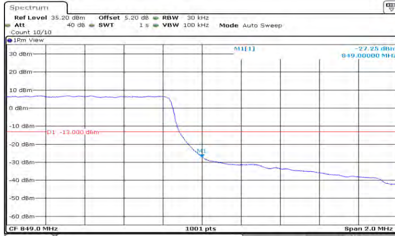
Band 26_1.4MHz_16QAM_27033_6RB#0
