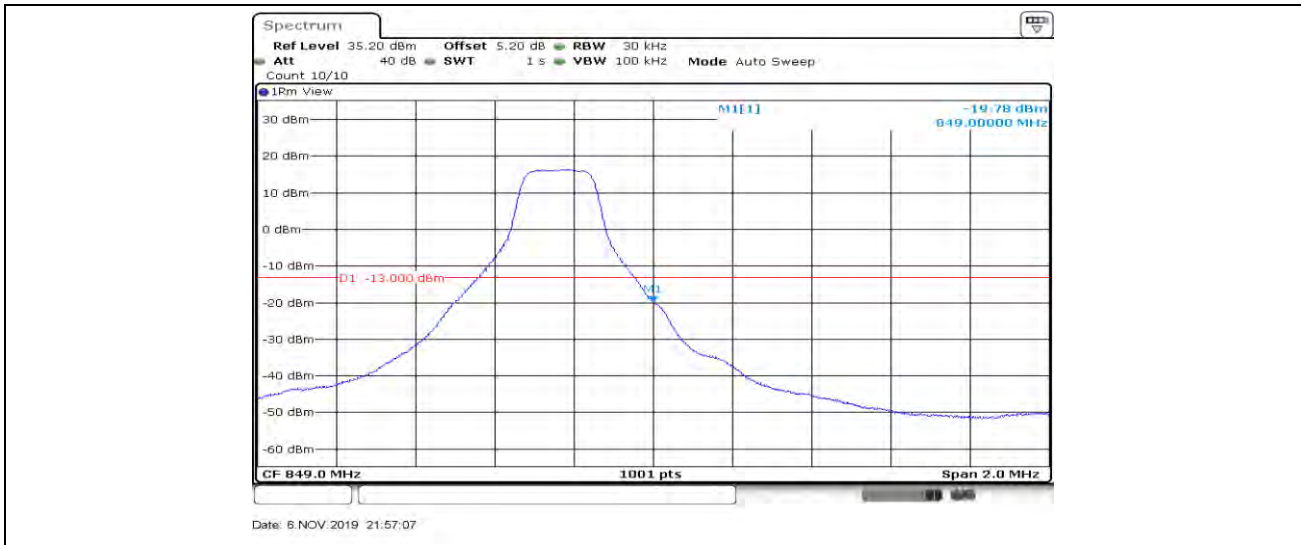
Band 26_3MHz_QPSK_27025_15RB#0
