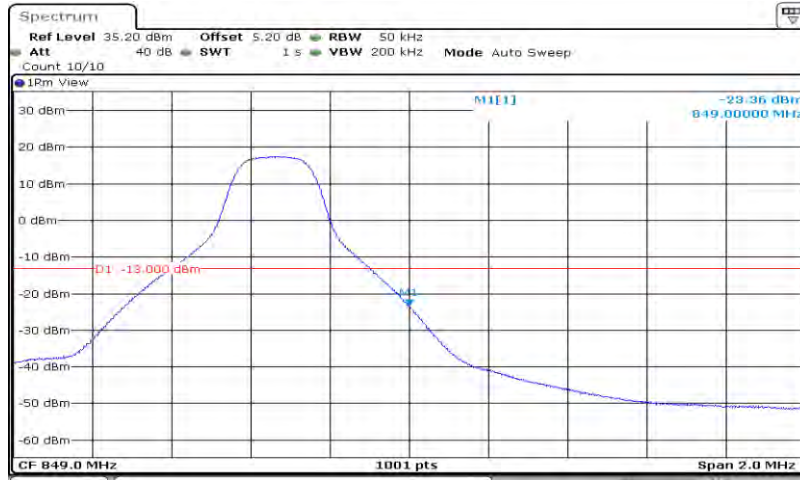
Band 26_5MHz_16QAM_27015_25RB#0
