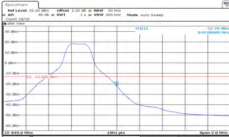
Band 26_5MHz_QPSK_27015_25RB#0
