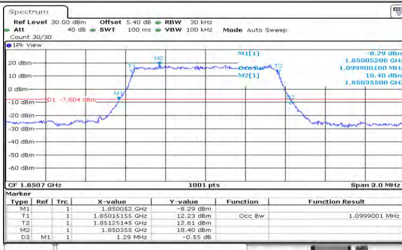
Band25-1.4MHz-QPSK-26047-6RB#0-1.1
