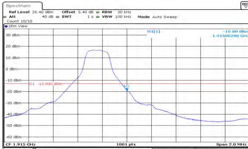
Band25-3MHz-QPSK-26675-15RB#0
