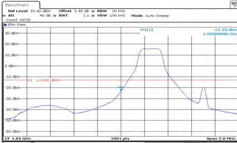
Band25-1.4MHz-16QAM-26047-6RB#0
