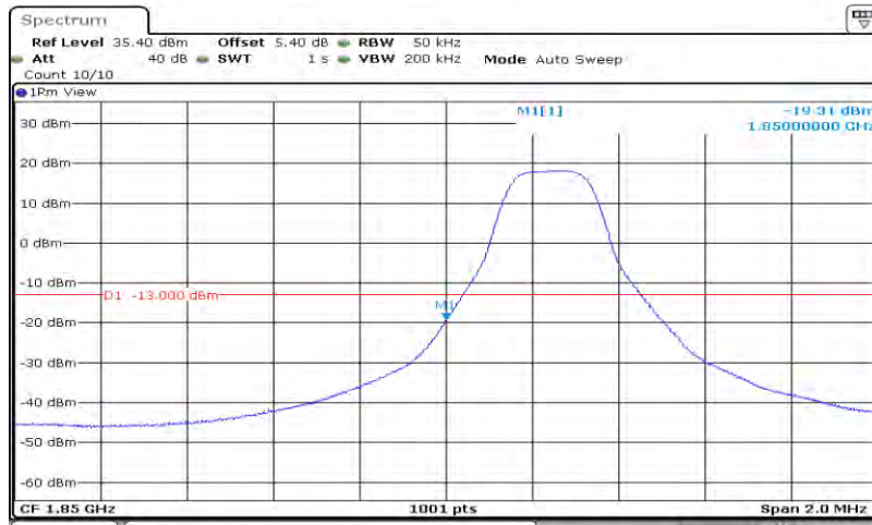
Band25-3MHz-16QAM-26055-15RB#0
