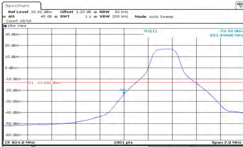
Band5-5MHz-16QAM-20425-25RB#0
