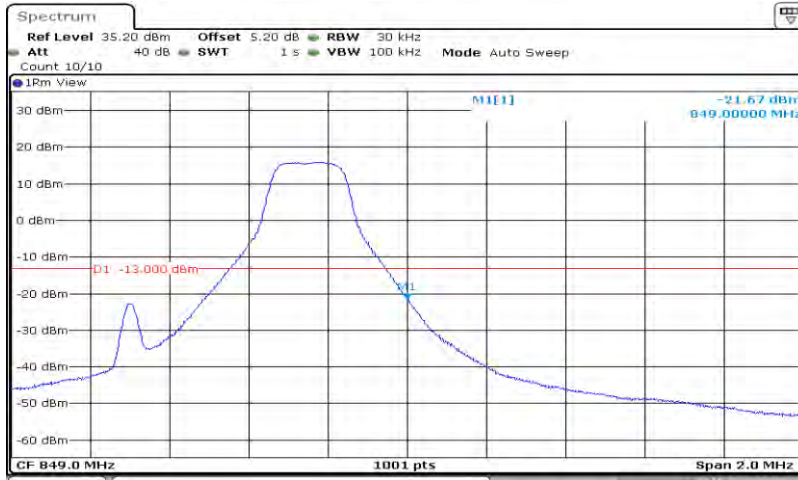
Band5-1.4MHz-16QAM-20643-6RB#0
