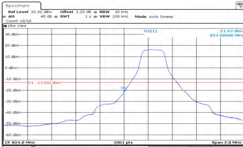
Band5-3MHz-QPSK-20415-15RB#0
