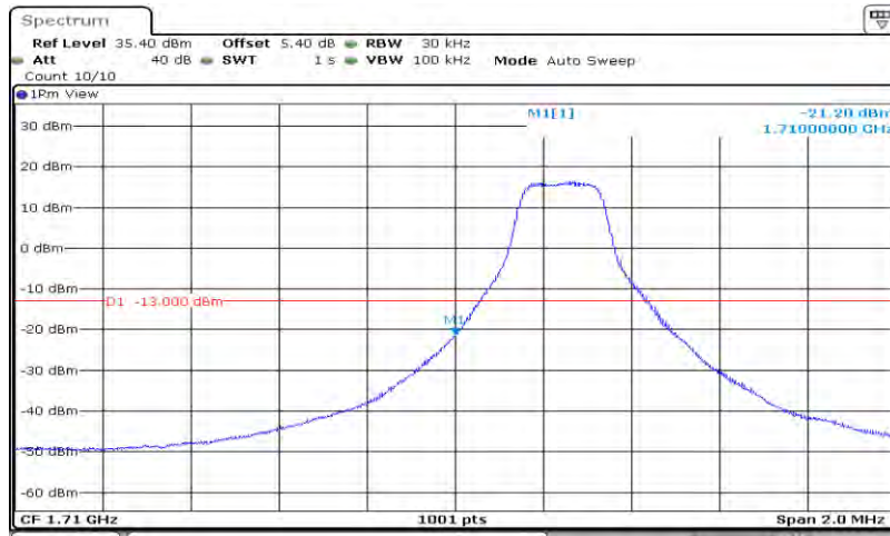
Band4-3MHz-16QAM-19965-15RB#0
