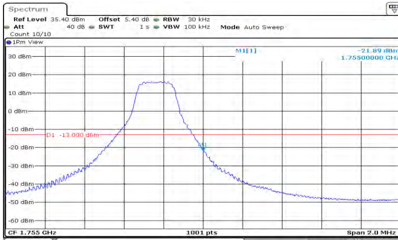
Band4-3MHz-16QAM-20385-15RB#0
