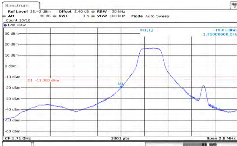
Band4-1.4MHz-16QAM-19957-6RB#0
