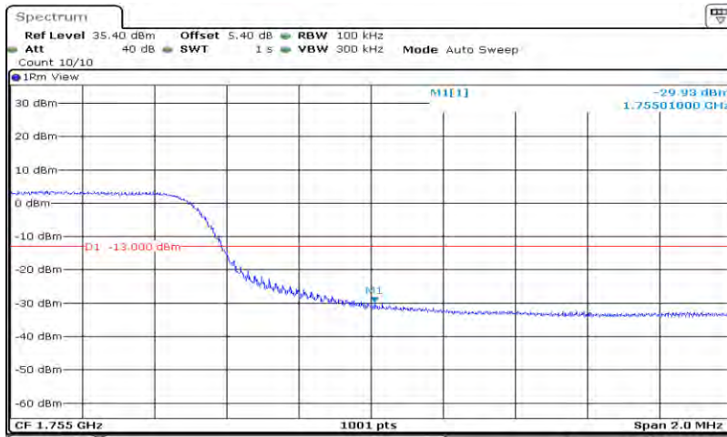
Band4-10MHz-16QAM-20350-50RB#0
