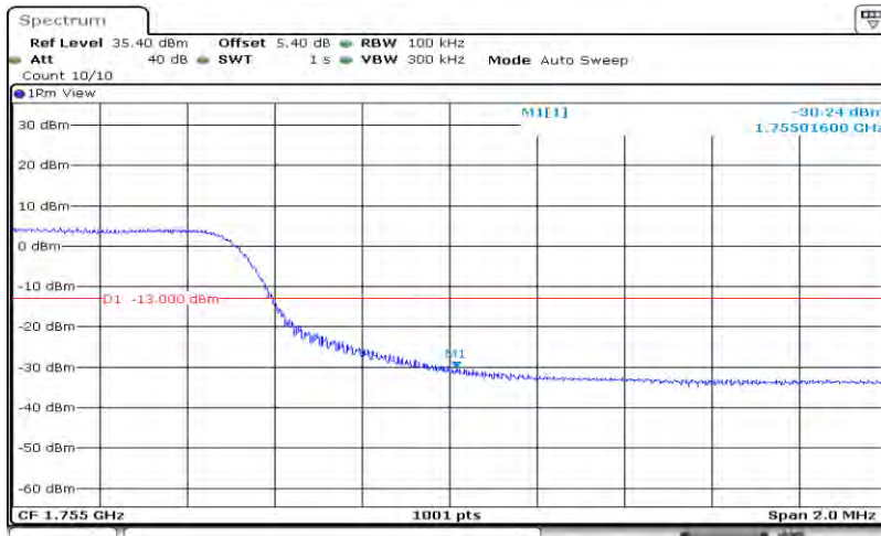
Band4-10MHz-QPSK-20350-50RB#0
