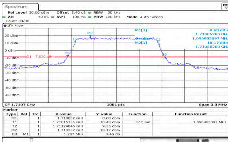
Band4-1.4MHz-QPSK-19957-6RB#0-1.097
