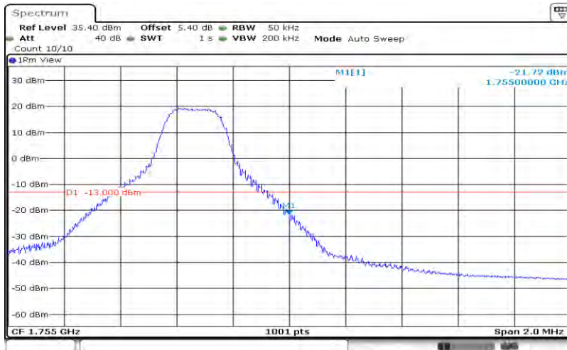
Band4-5MHz-QPSK-20375-25RB#0
