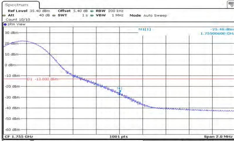
Band4-15MHz-16QAM-20325-75RB#0
