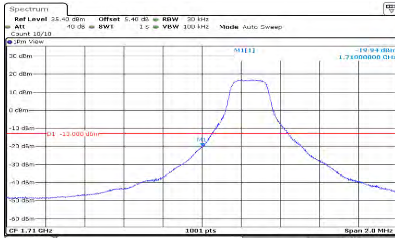
Band4-3MHz-QPSK-19965-15RB#0
