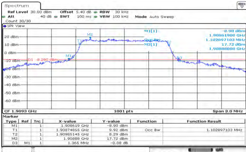
Band2-1.4MHz-16QAM-19193-6RB#0-1.103
