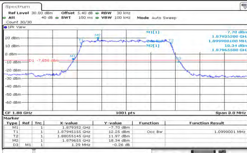
Band2-1.4MHz-QPSK-18900-6RB#0-1.1
