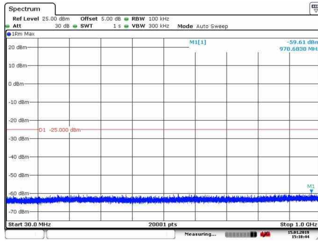
Band41_20MHz_16QAM_40620_1RB#0
