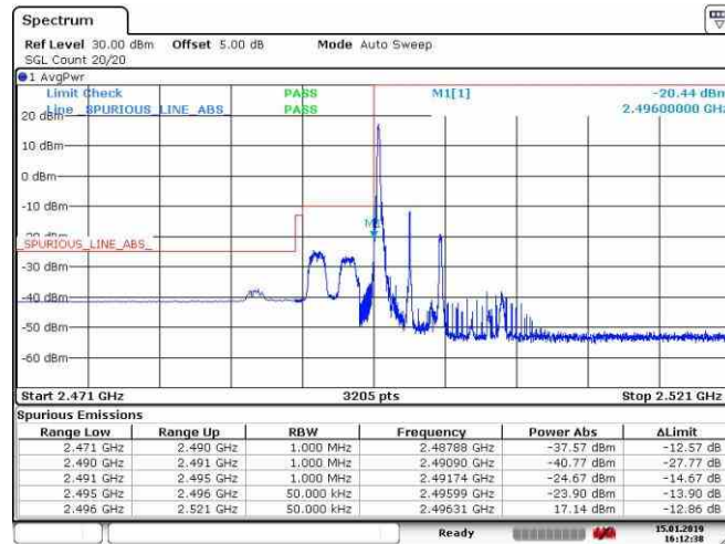
BAND 41_5MHz_QPSK_39675_1RB#0
