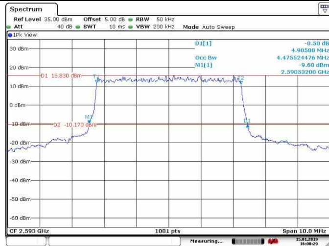
Band41_5MHz_16QAM_40620_25RB#0
