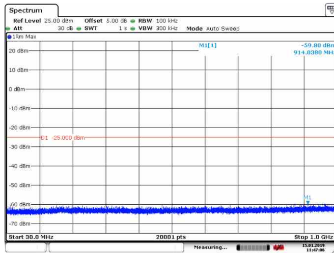
Band41_20MHz_16QAM_41490_1RB#0
