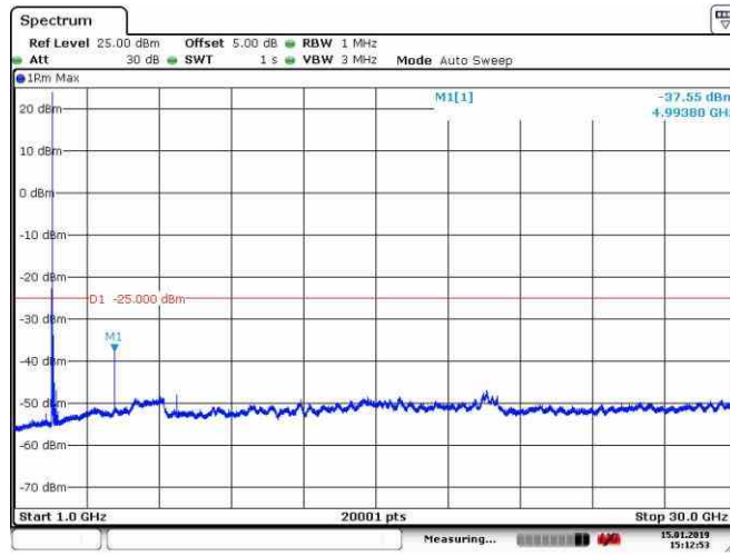
Band41_20MHz_16QAM_39750_1RB#0
