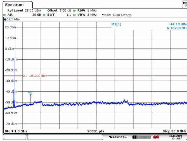
Band41_20MHz_16QAM_40620_1RB#0
