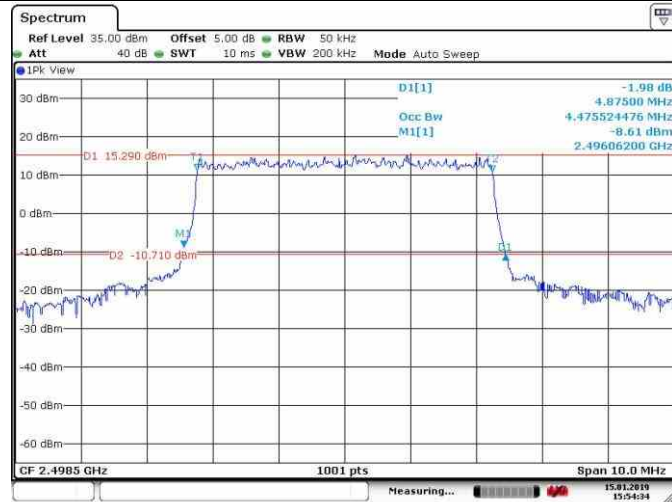
Band41_5MHz_16QAM_39675_25RB#0
