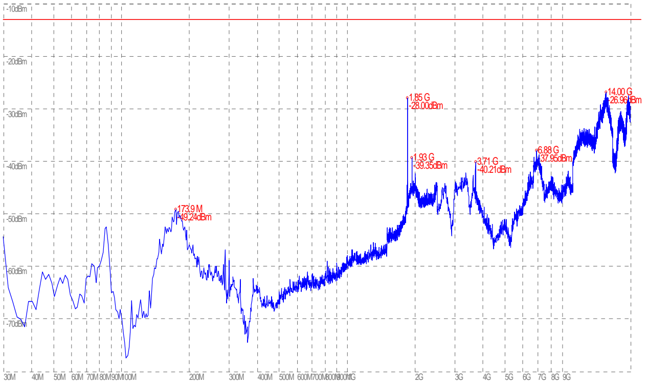
(Plot H.2: HSDPA 1900 MHz Channel = 9262, Test Antenna Vertical)
