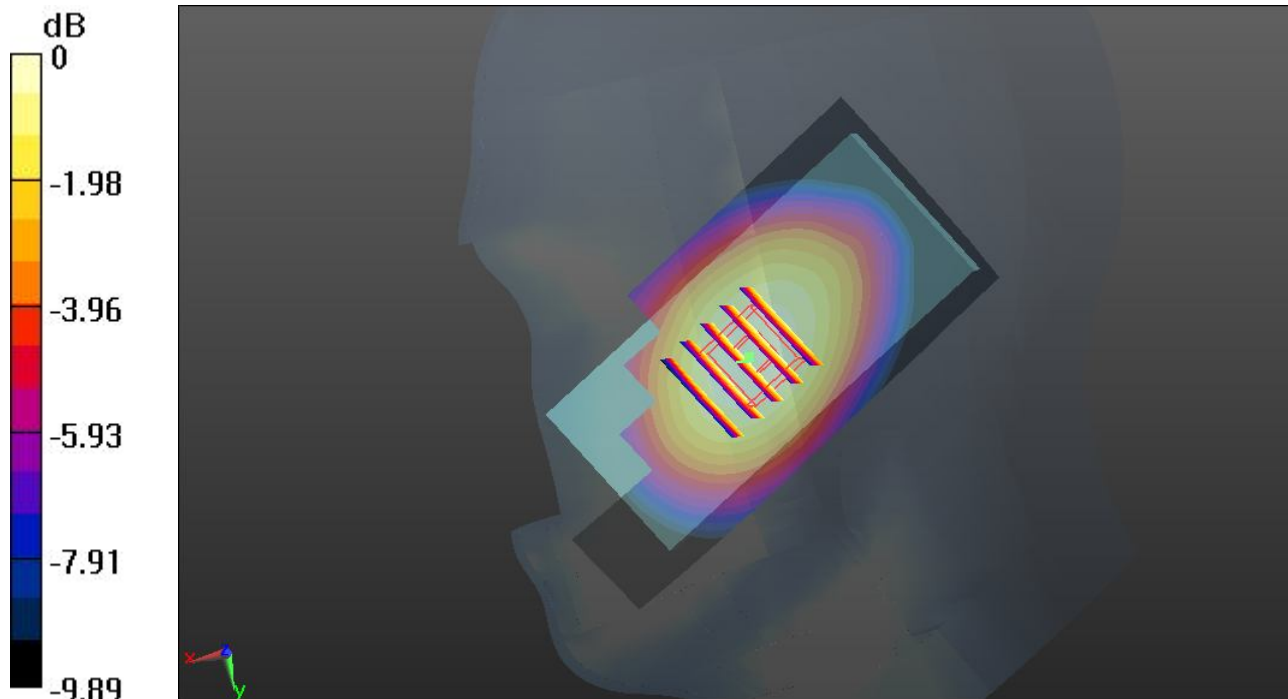
0 dB = 0.492 W/kg
