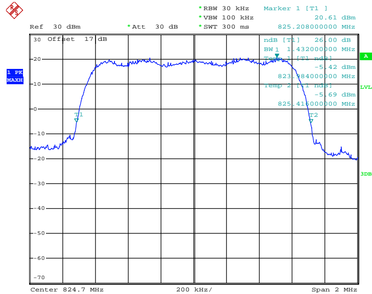
26dB Bandwidth Plot on Channel 1013 (824.70 MHz)
