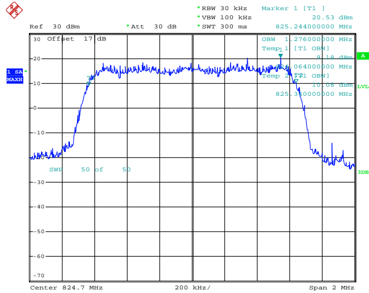
99% Occupied Bandwidth Plot on Channel 1013 (824.70 MHz)
