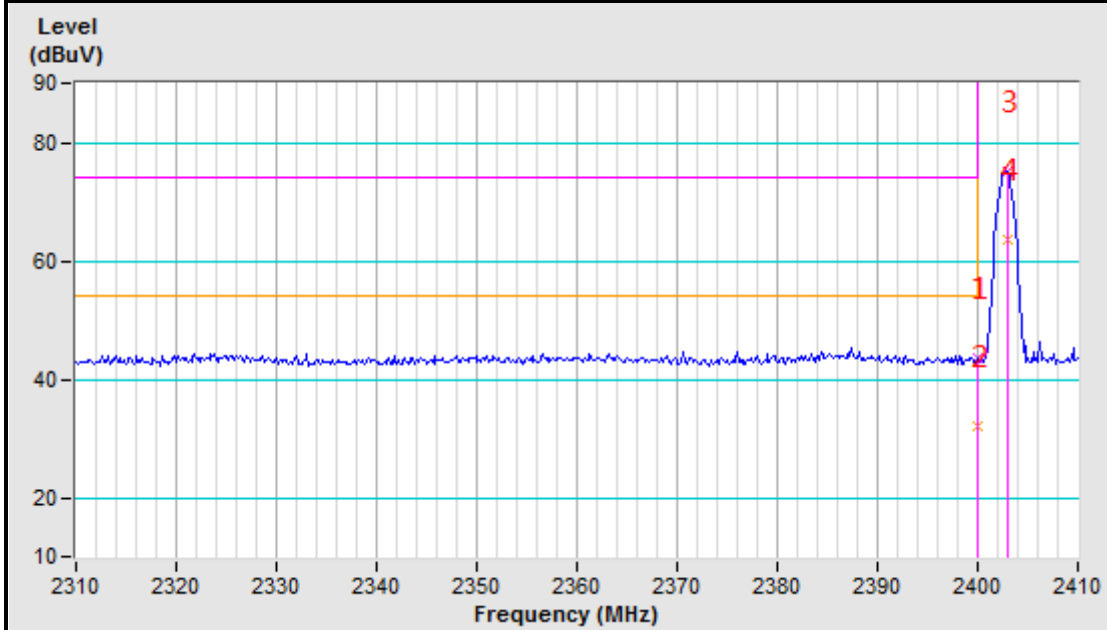
2403MHz Vertical
