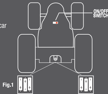
BOTTOM SIDE: FLIP OVER AND INSERT 3 "AA" BATTERIES IN THE POLARITY DIRECTION SHOWN ON THE BOTTOM SIDE
