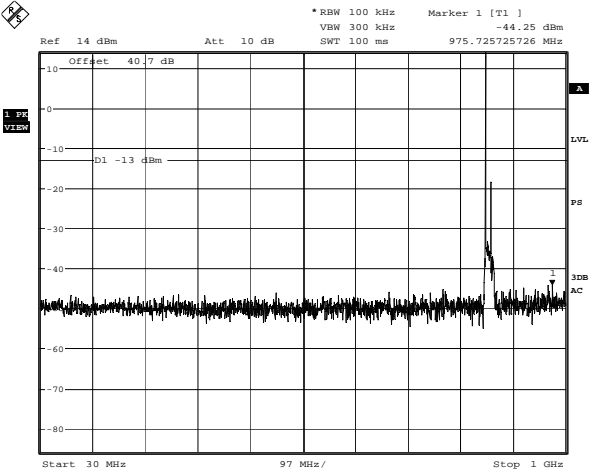
Downlink - 4FSK - Low Channel - Conducted Emissions Date: 9.NOV.2006 16:12:56
