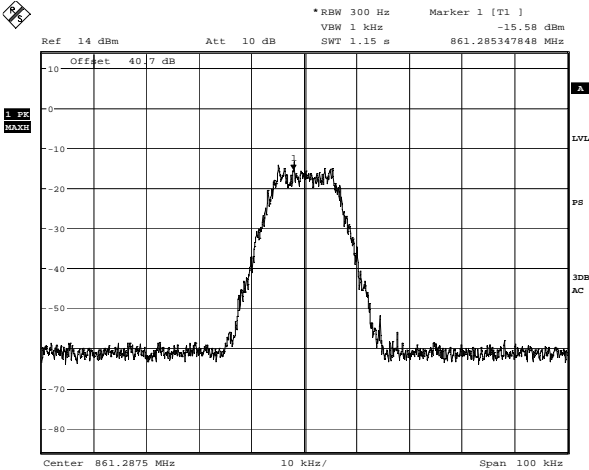
Downlink - 4FSK Output Date: 9.NOV.2006 15:14:30
