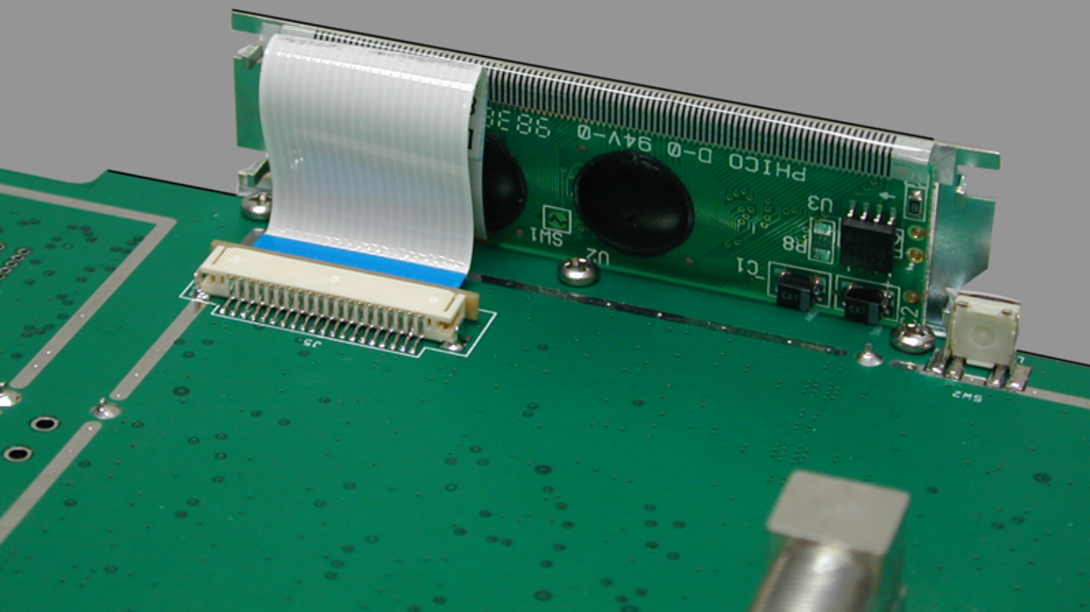
SCU - INTERNAL REAR VIEW OF LCD DISPLAY
