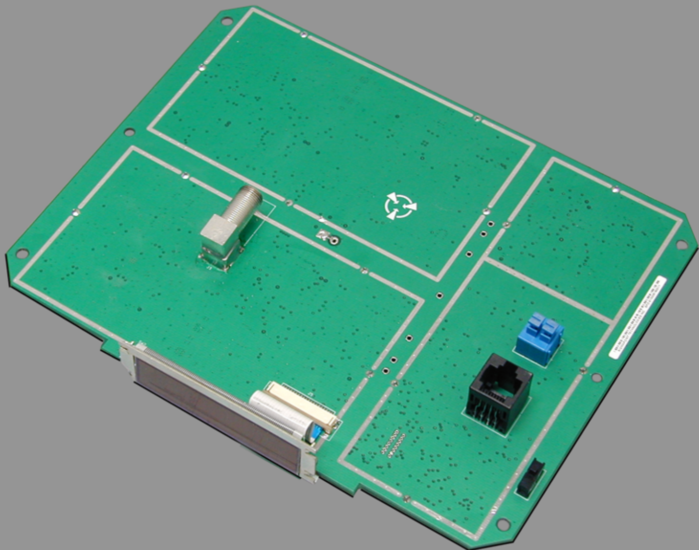
SCU - INTERNAL VIEW OF TRACK SIDE RADIO CIRCUITRY
