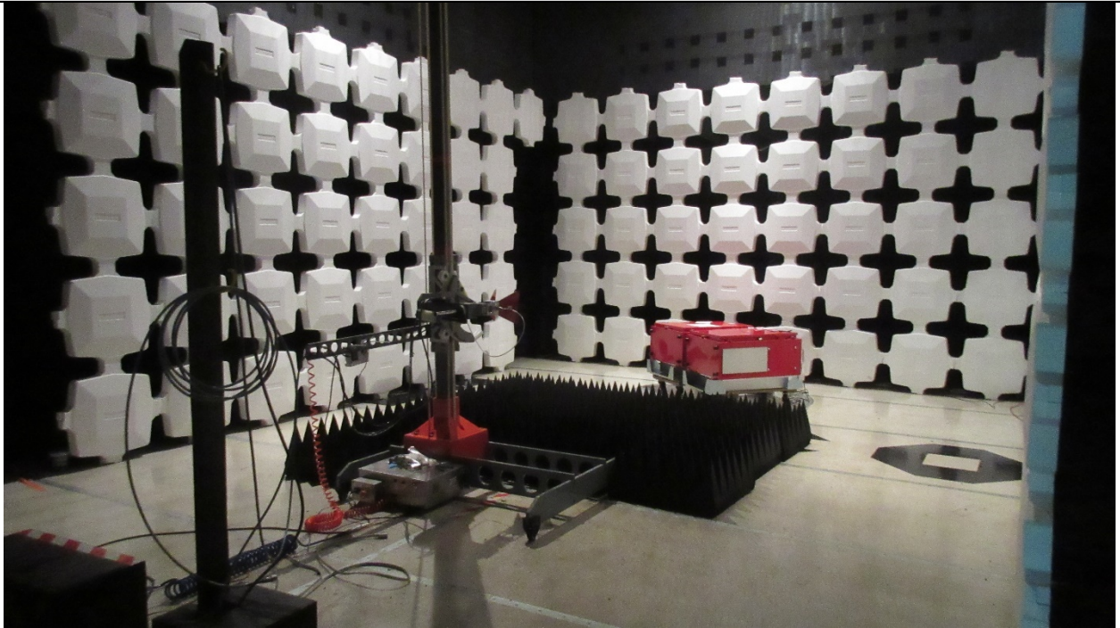
Testing, Above 1 GHz at 1m
