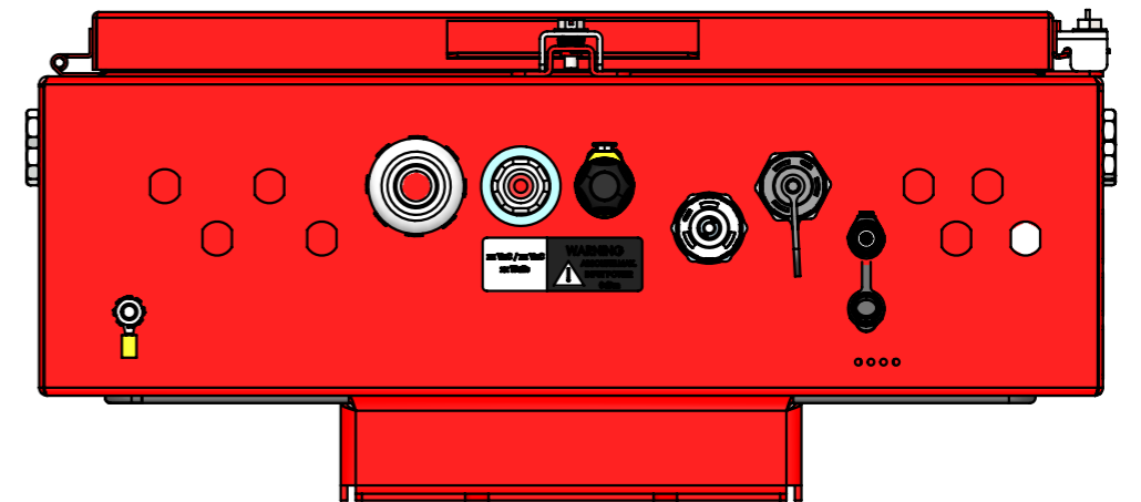
BOTTOM VIEW
