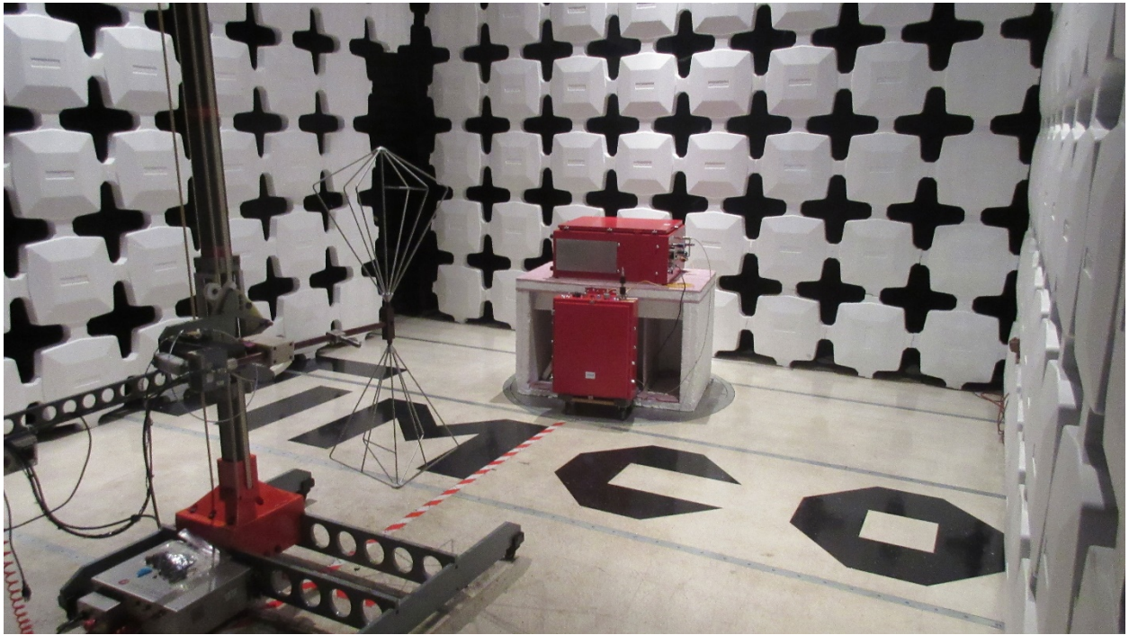
Radiated, Below 1 GHz
