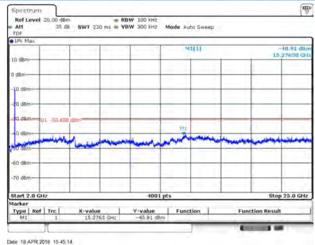
802.11n-40 MHz LOW CHANNEL, SPURIOUS 2 GHz ~ 25 GHz
