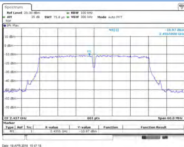
802.11n-40 MHz MIDDLE CHANNEL CARRIER LEVEL
