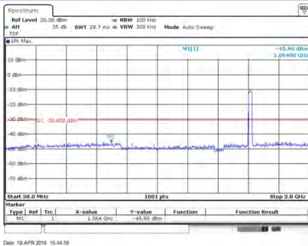
802.11n-40 MHz LOW CHANNEL, SPURIOUS 30 MHz ~ 3 GHz
