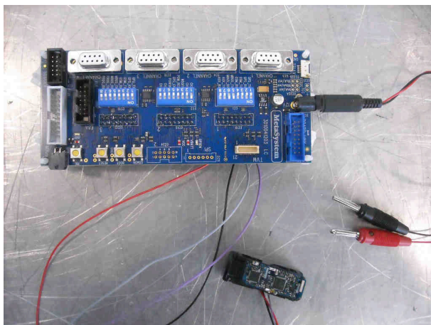
Test JIG
