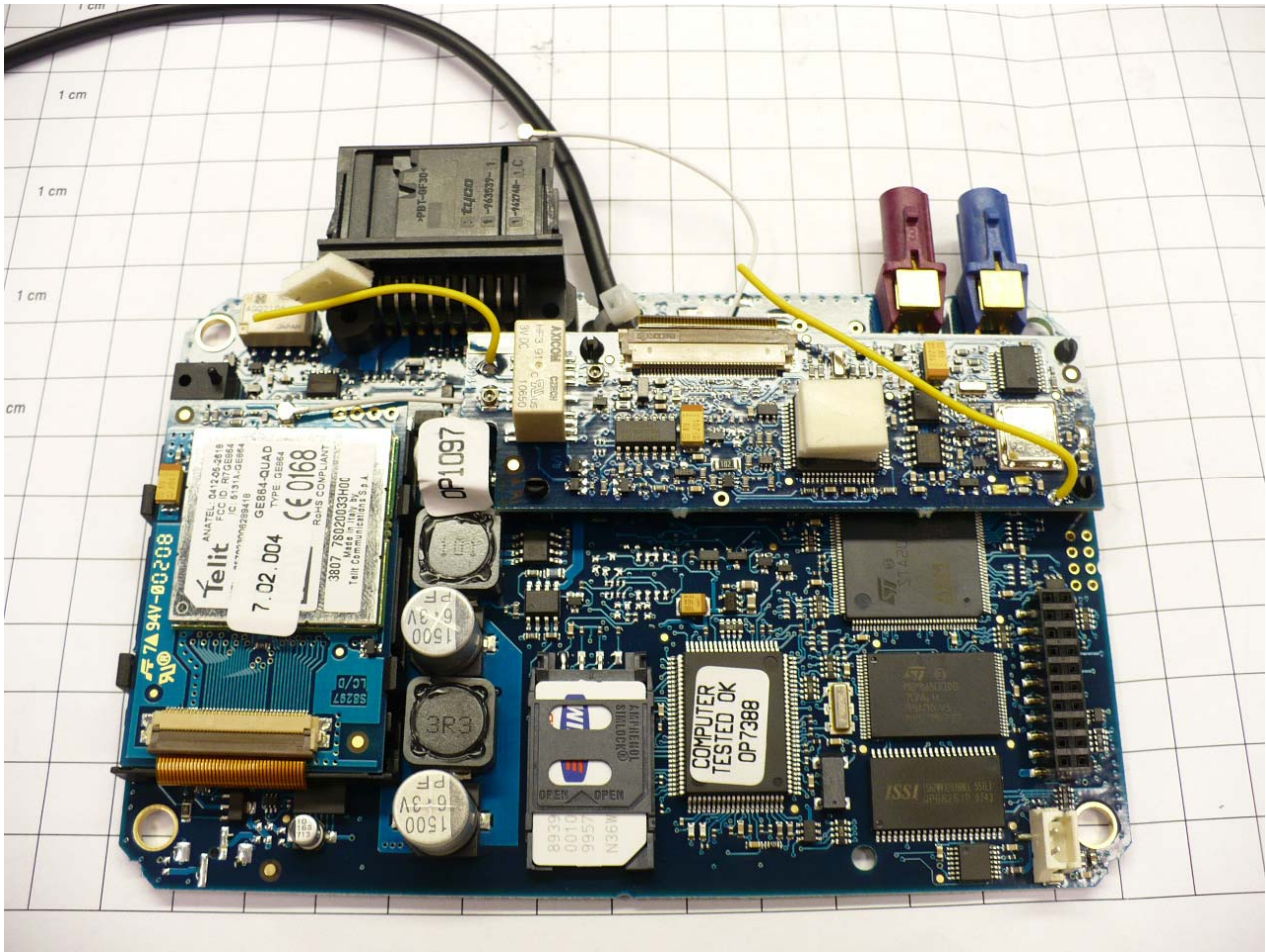
FRONT WIEV
