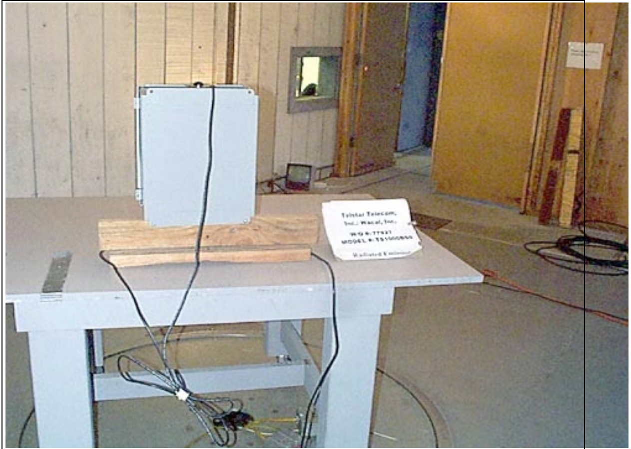
Radiated Emissions - Back View of Base Station
