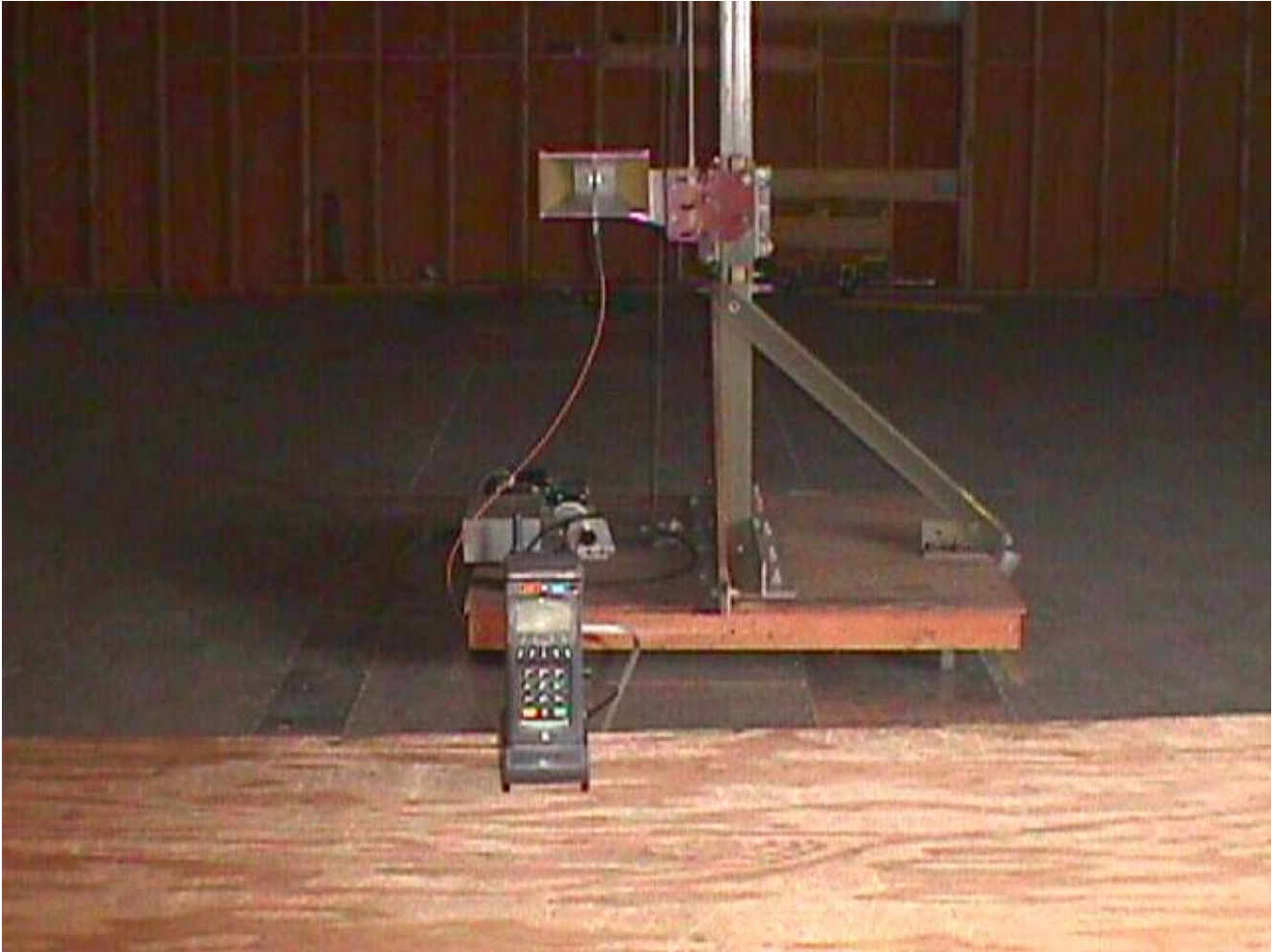
Radiated Emissions at 3 Meters Distance
