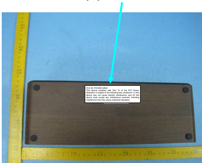
Proposed Label Location on EUT EUT Bottom View/ proposed FCC Label Location
