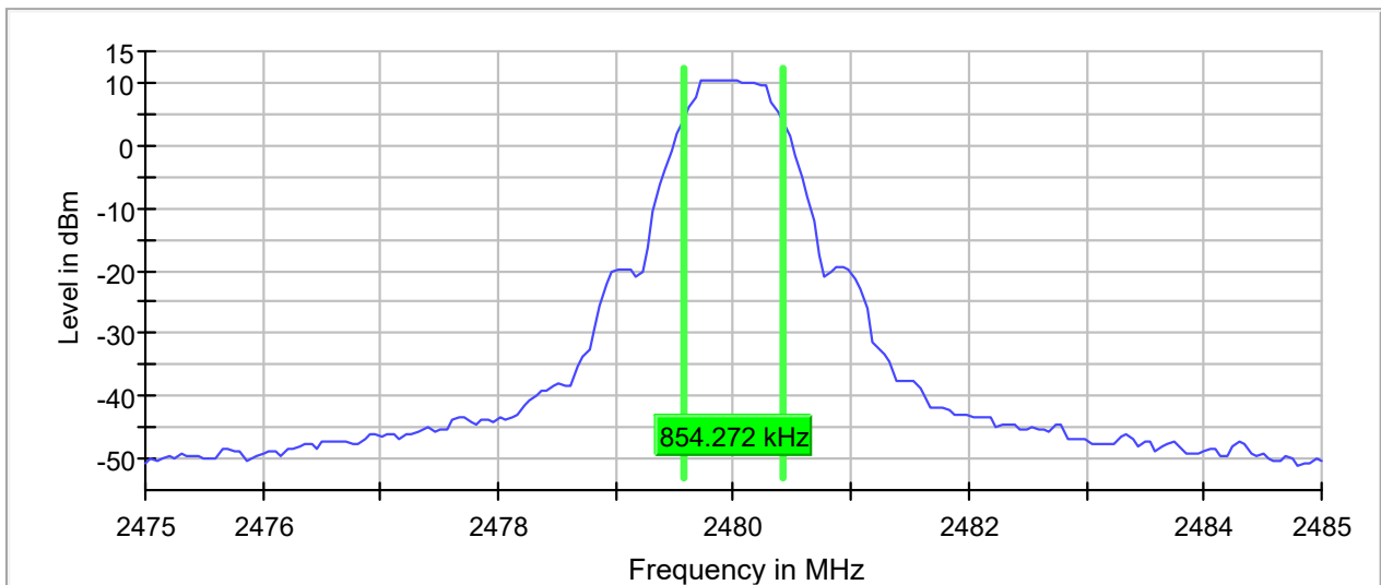
6 dB Bandwidth
