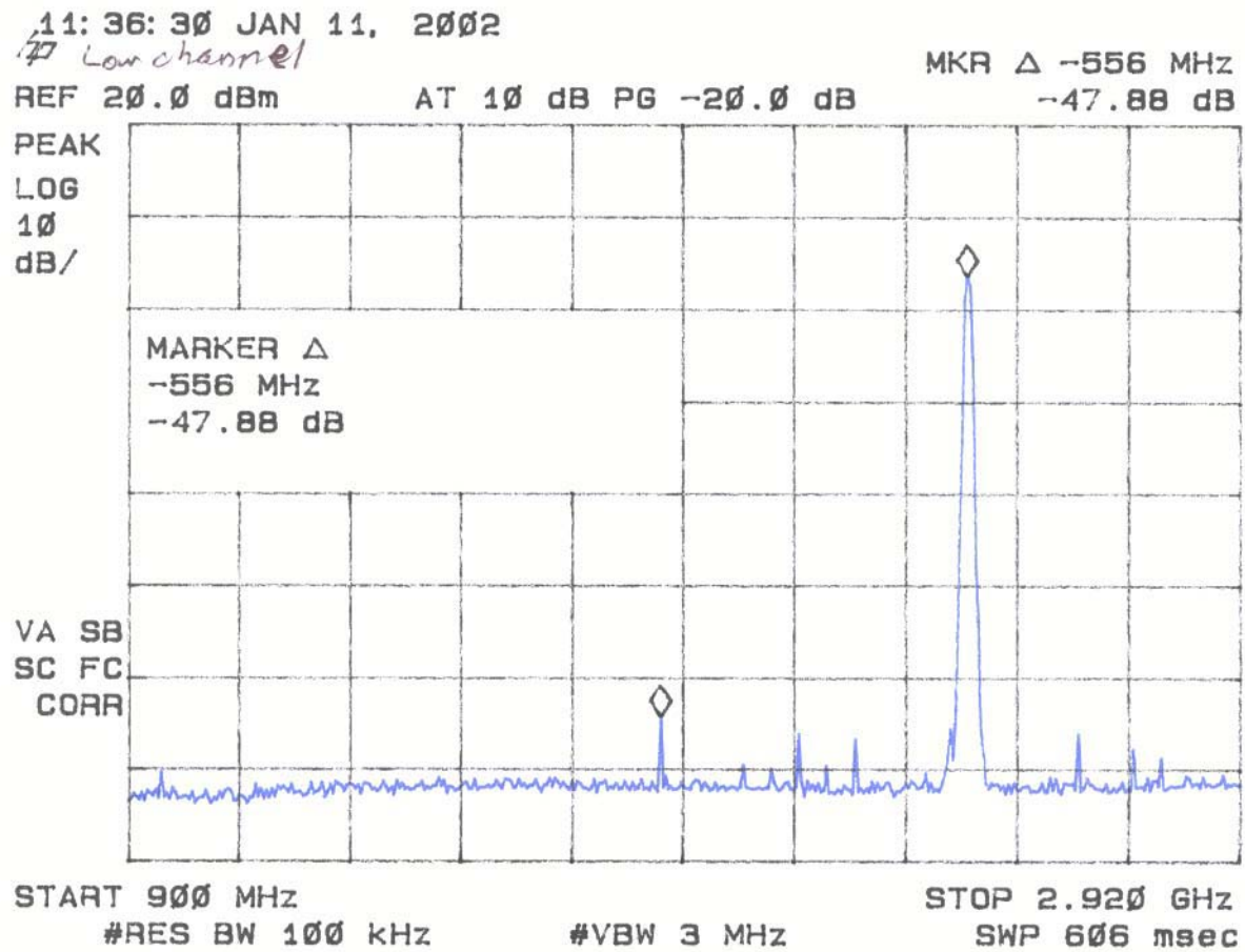
Figure 4b Antenna Conducted Spurious Emissions 5.247(c) Low
