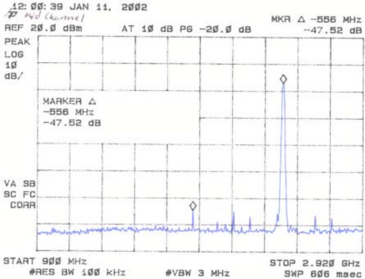
Figure 4f Antenna Conducted Spurious Emissions 15.247(c) Mid
