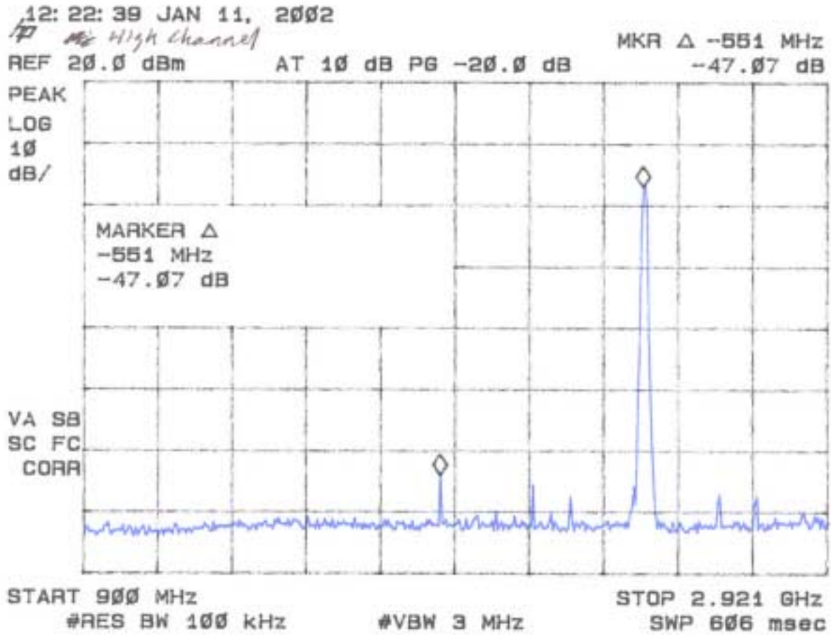
Figure 4j Antenna Conducted Spurious Emissions 15.247(c) High
