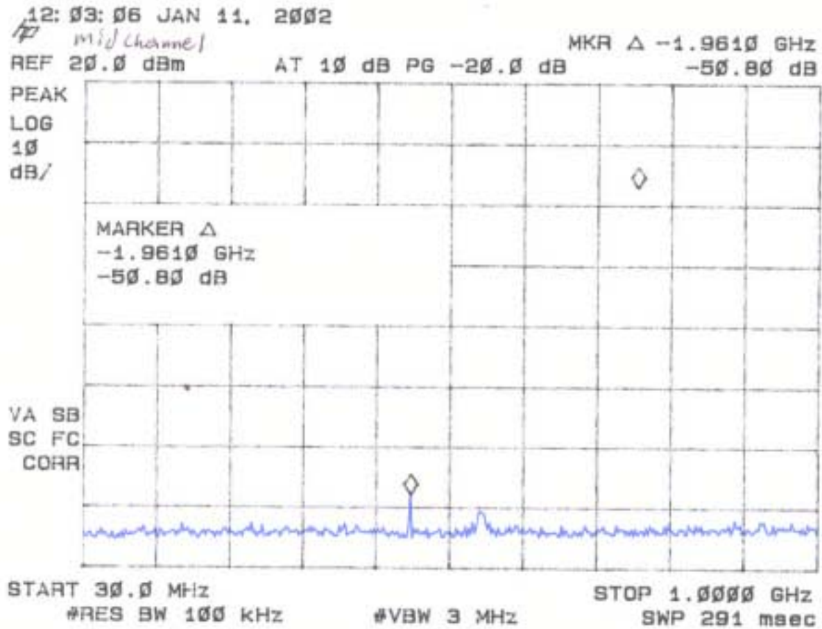
Figure 4e Antenna Conducted Spurious Emissions 15.247(c) Mid
