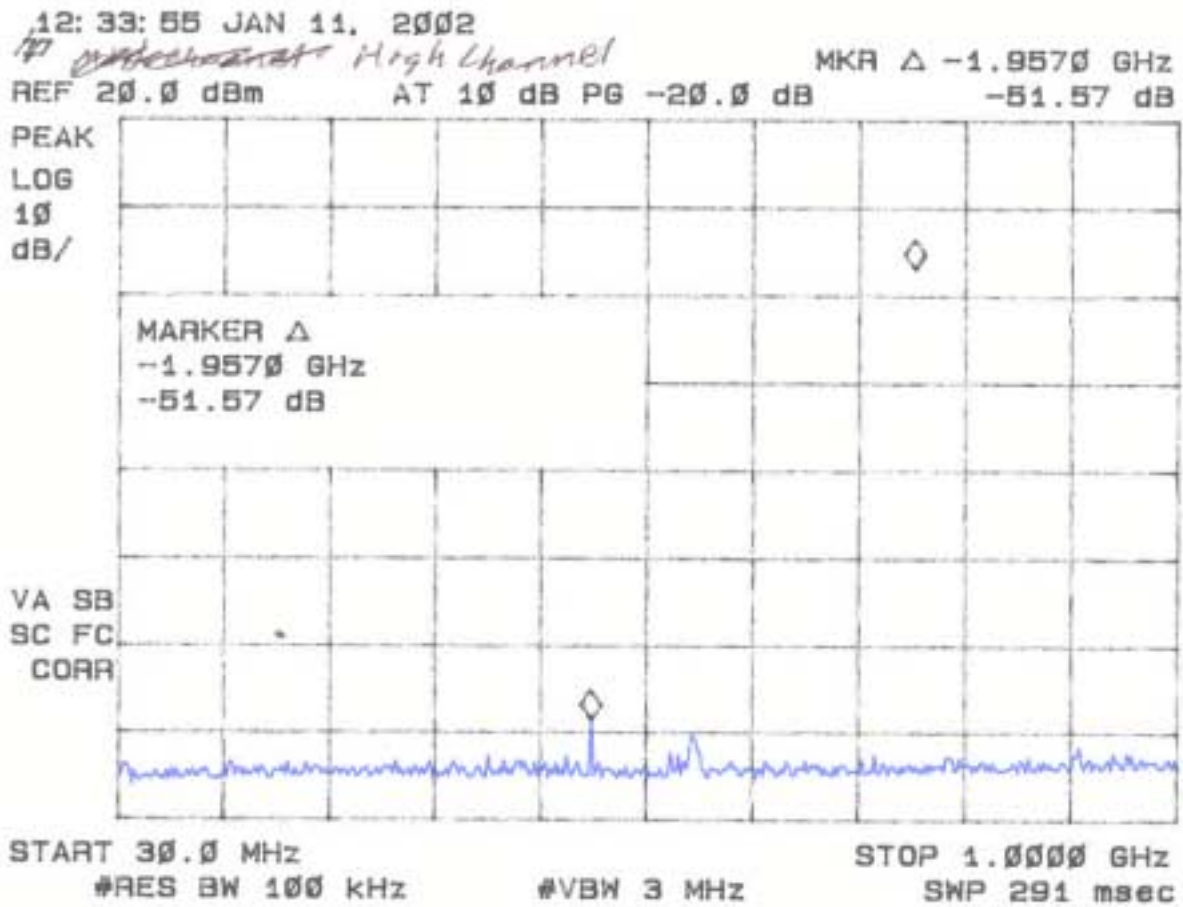
Figure 4i Antenna Conducted Spurious Emissions 15.247(c) High
