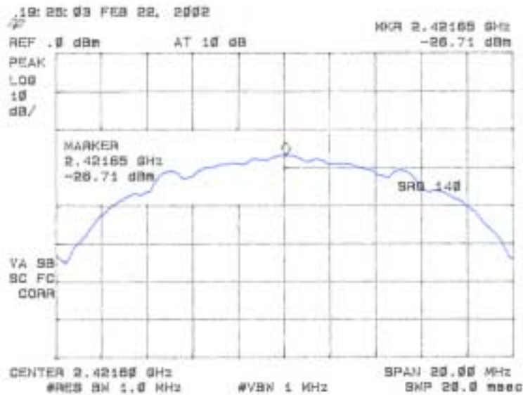
Figure 6g Bandedge Plots
