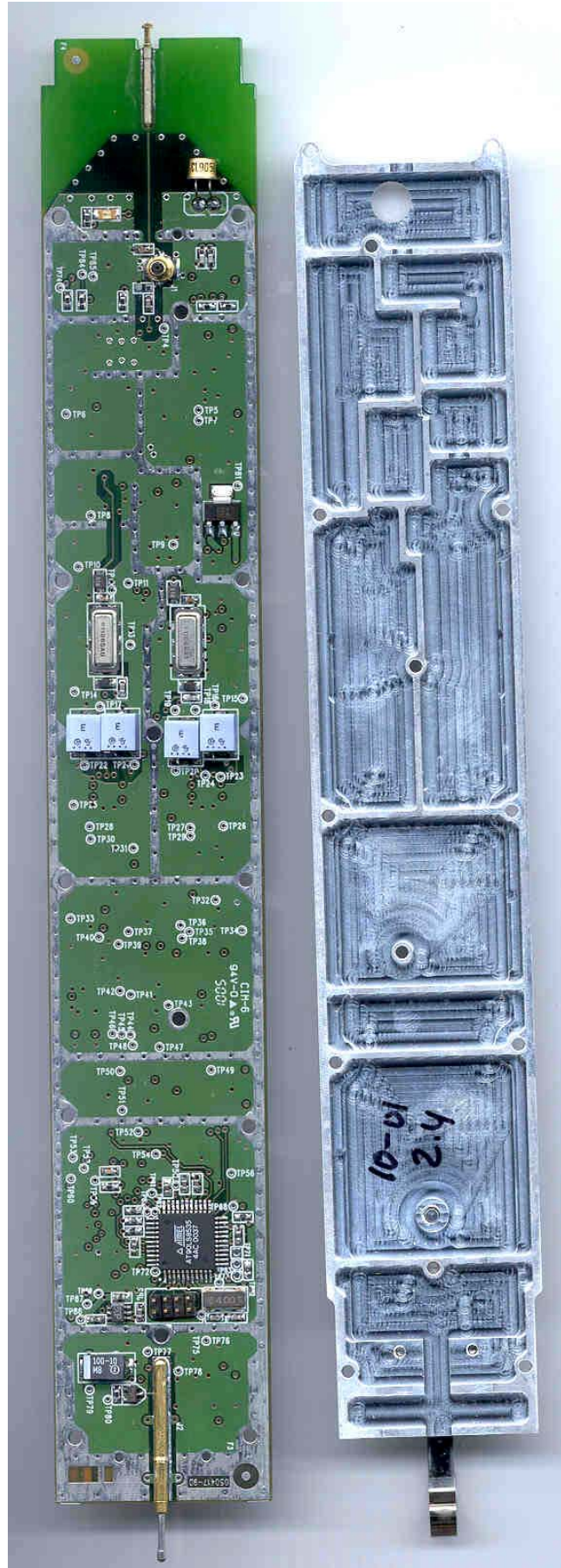
Photo 5. Top View - Cover Removed
