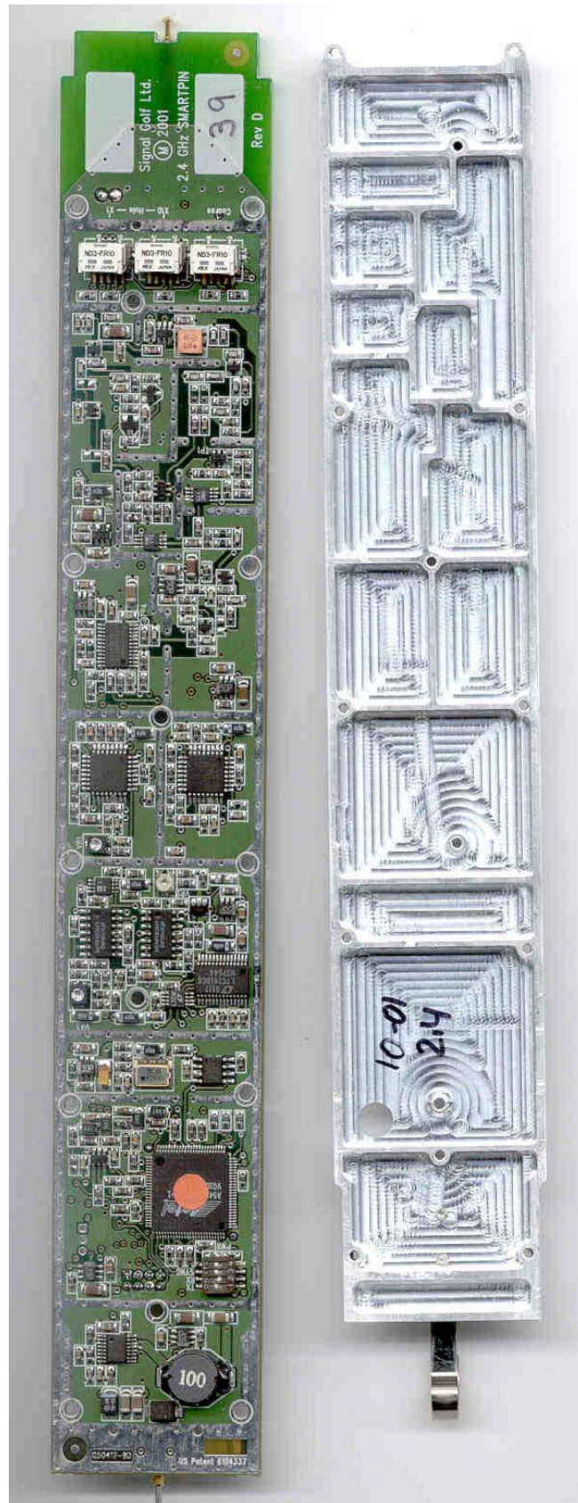
Photo 6. Bottom View - Cover Removed
