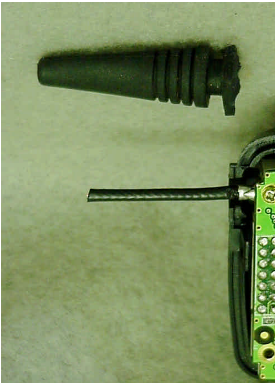
Photo 12. EUT, View of Antenna
