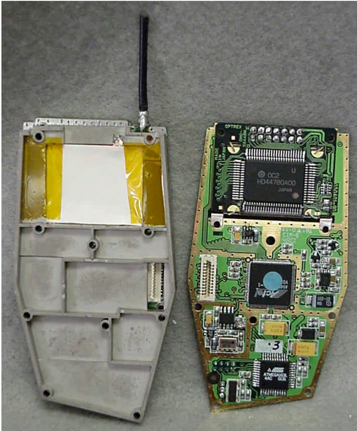
Photo 6. EUT, Bottom View of Board 1 & Shield
