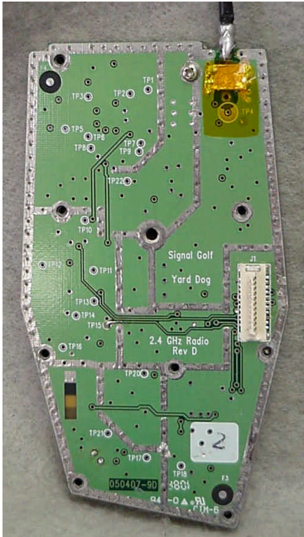
Photo 9. EUT, Top View of Board 2
