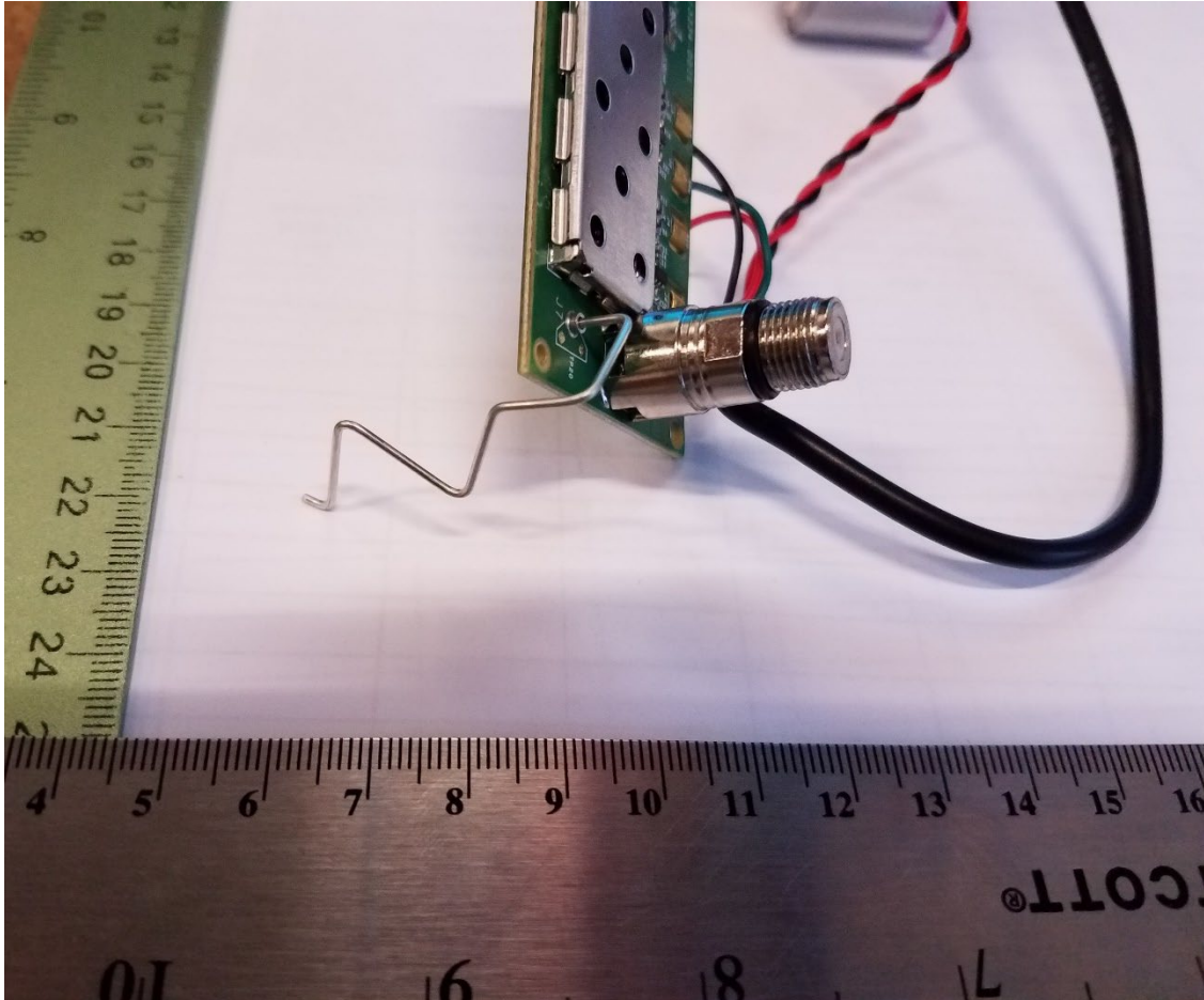
Figure 1. Monopole Antenna
