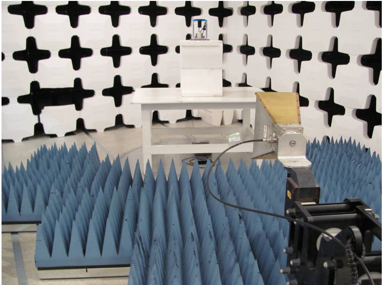
Figure 3. Radiated Emissions above 1 GHz
