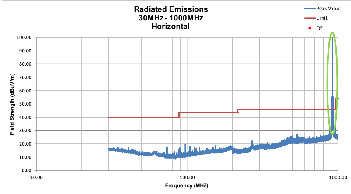
Figure 2. Radiated Emissions 30 MHz – 1000 MHz, Horizontal
