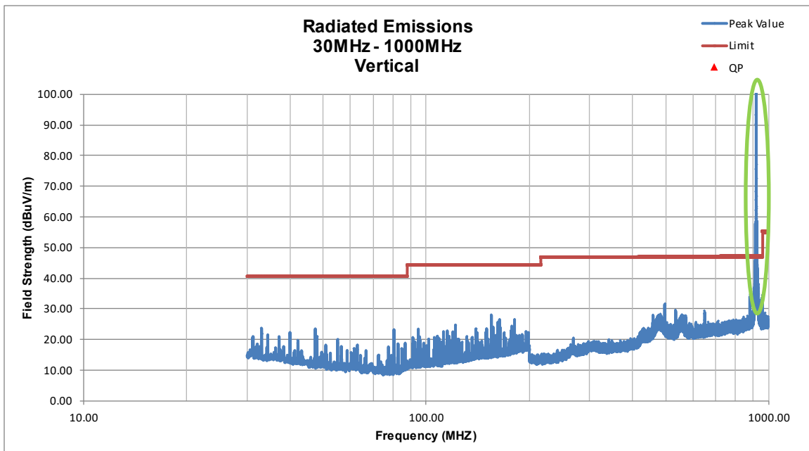
Figure 3. Radiated Emissions 30 MHz – 1000 MHz, Vertical
