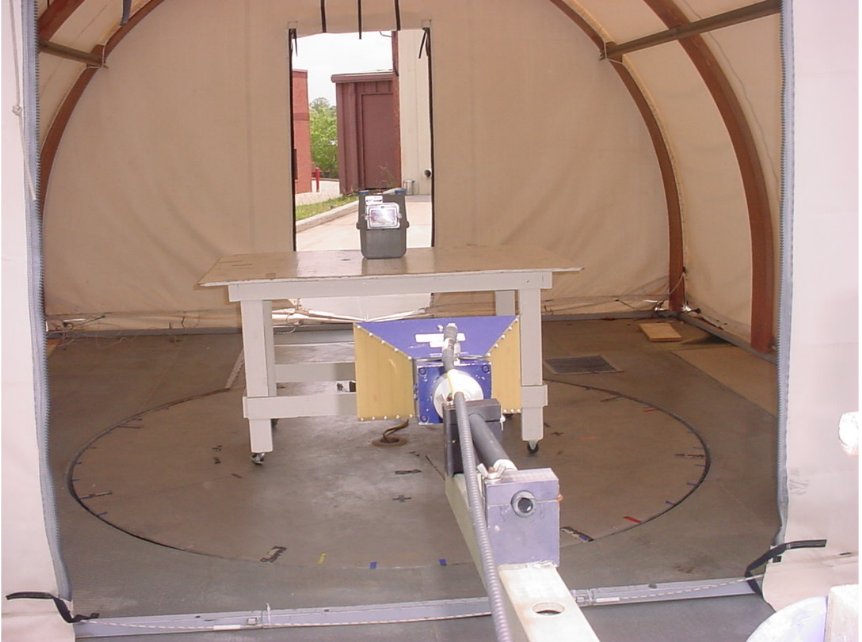
Figure 4: Test Setup – Radiated Emissions – Actaris Model Metris
