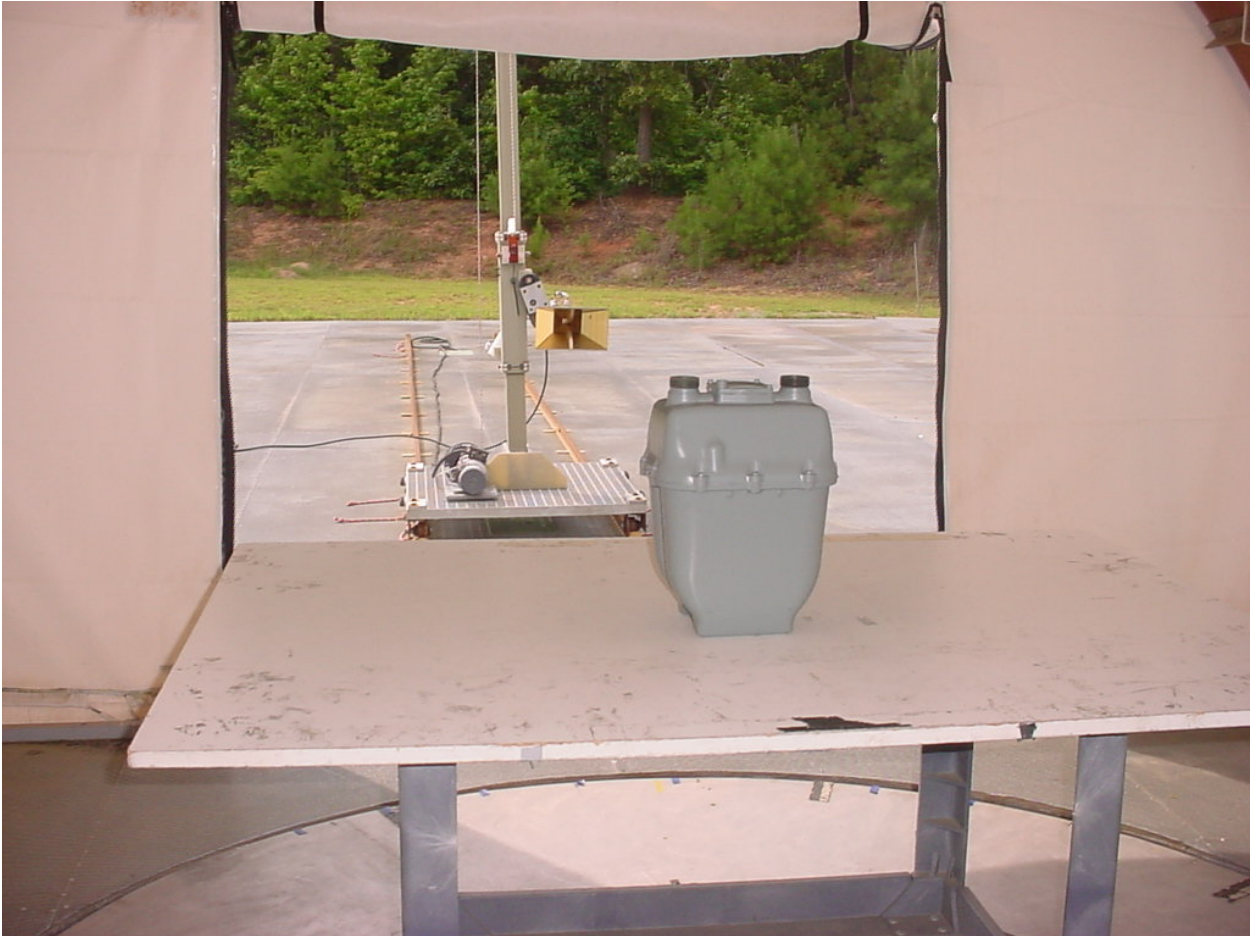
Figure 5: Test Setup – Radiated Emissions – Sensus Metering Systems Model R-275
