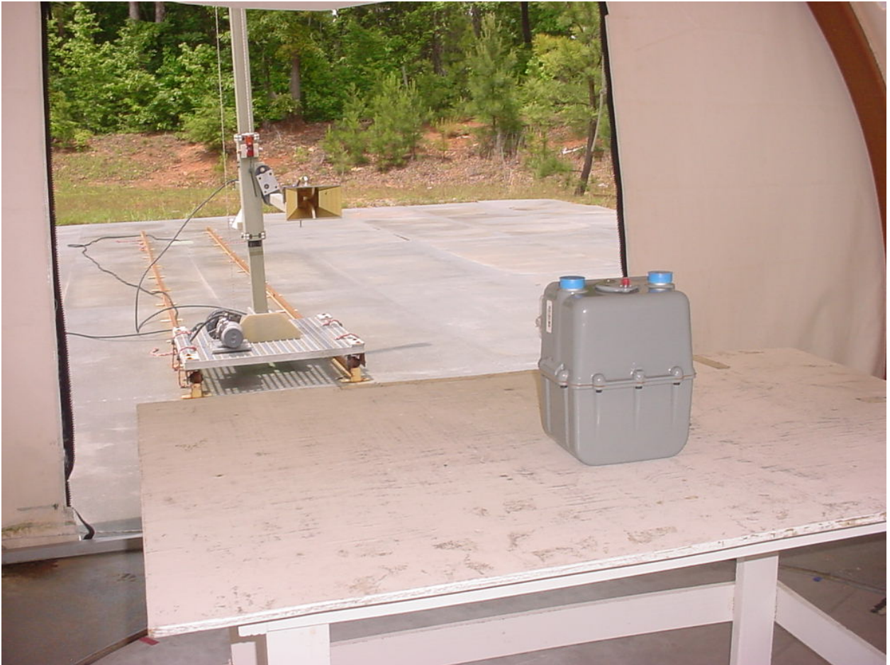
Figure 3: Test Setup – Radiated Emissions – Actaris Model Metris
