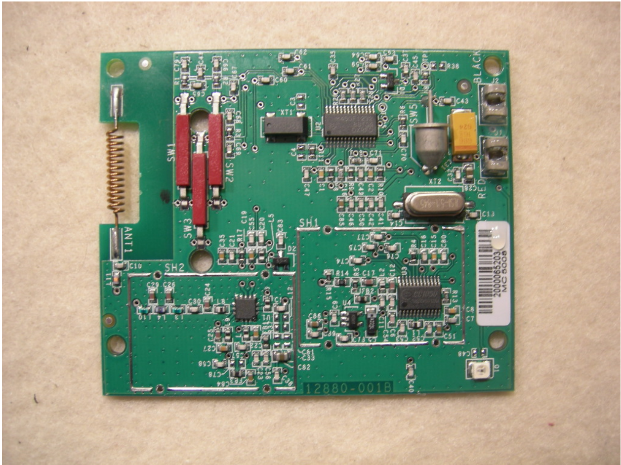
Figure 1: Front View without Shields
