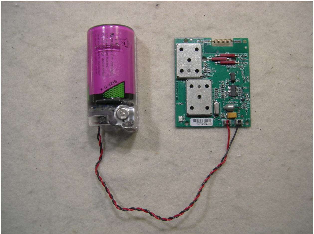
Figure 1: Front View w/ Battery
