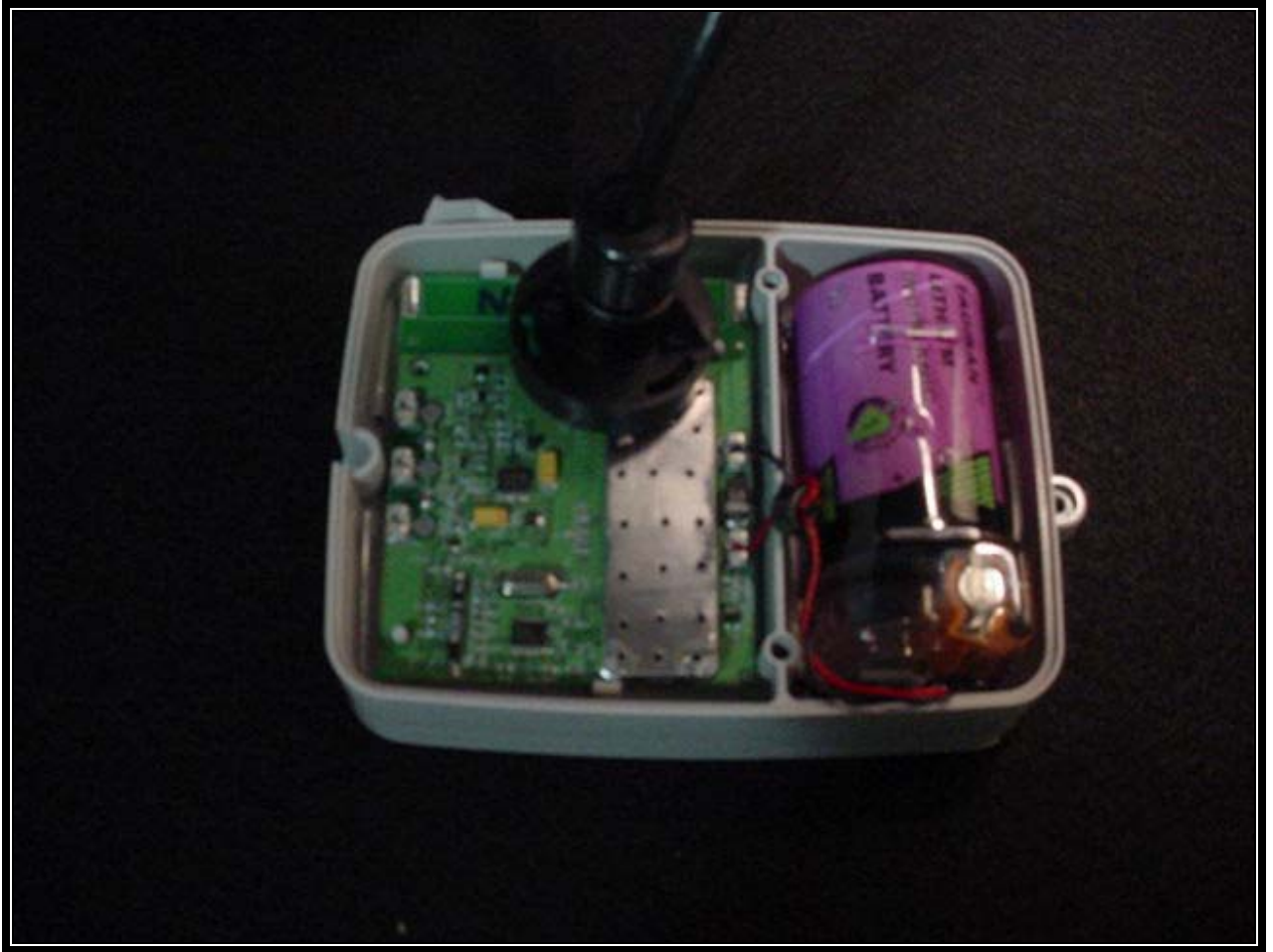
Figure C1: Pit Unit with Cover Off
