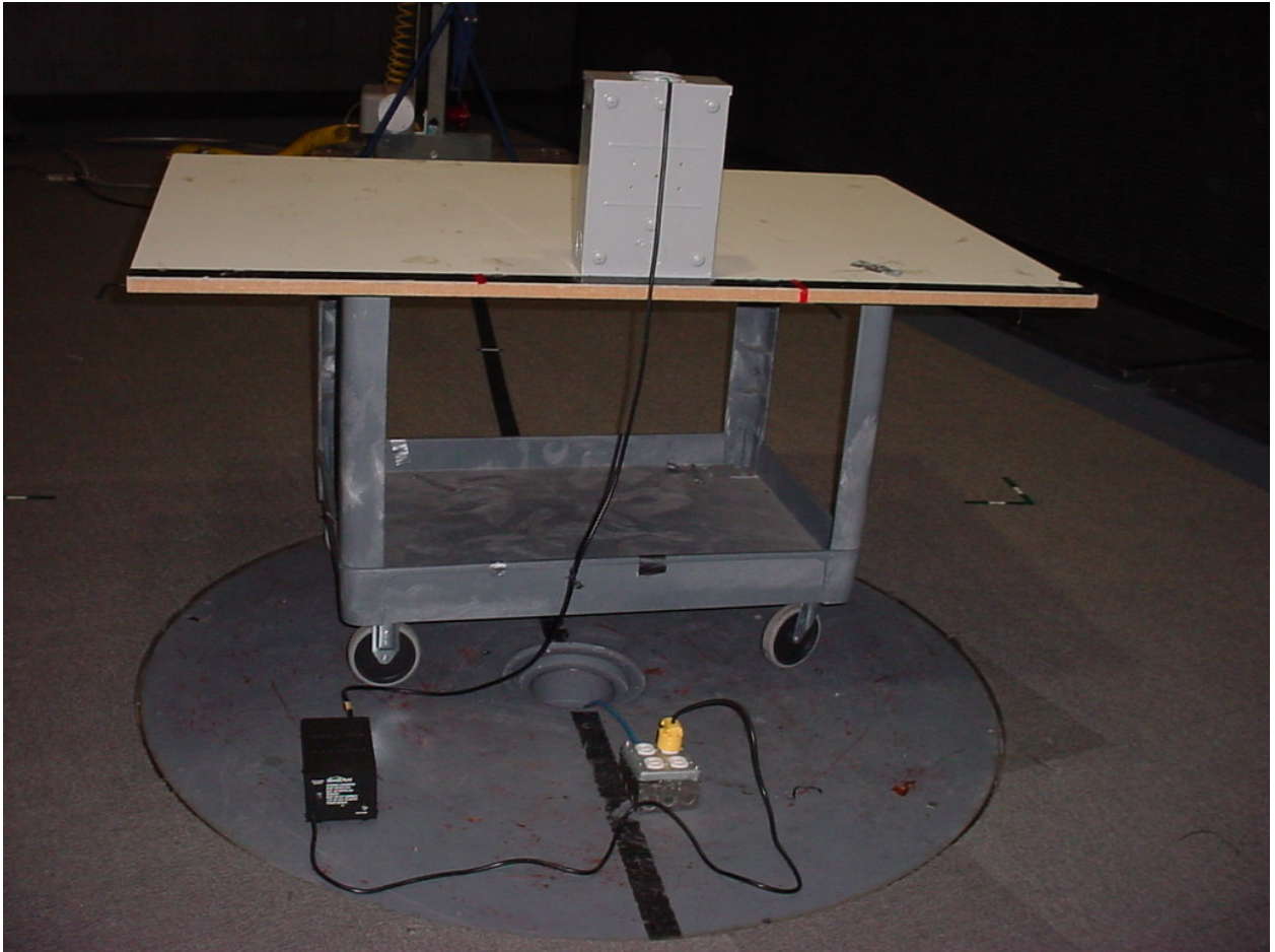
Figure 2: Test Setup – Radiated Emissions – Back View
