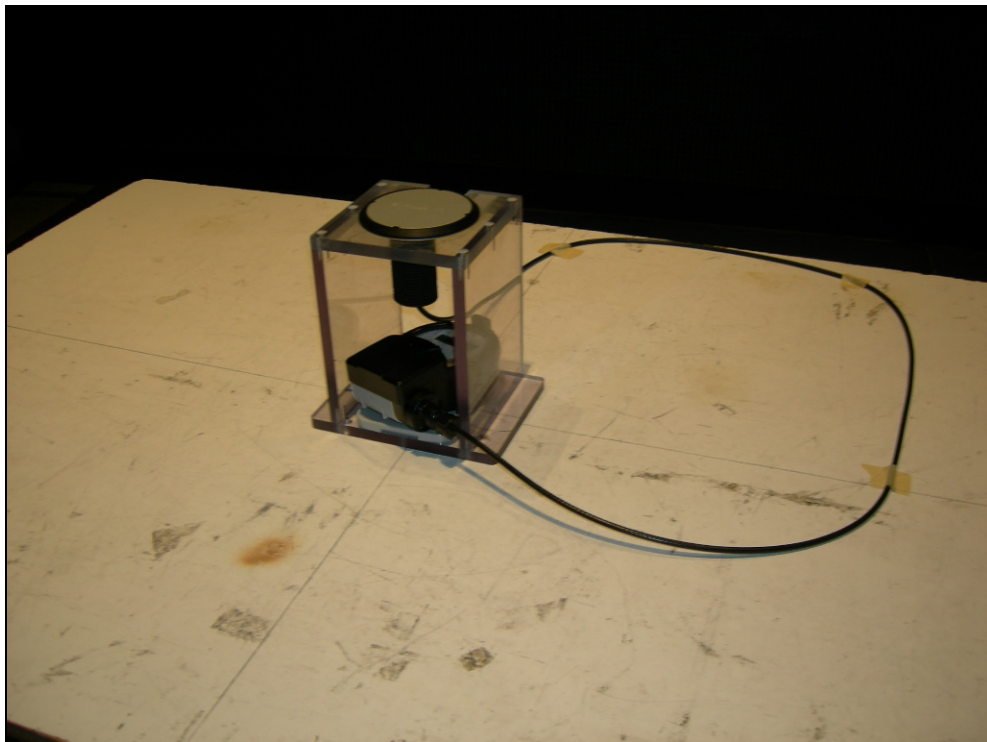
Figure 4: Radiated Emissions
