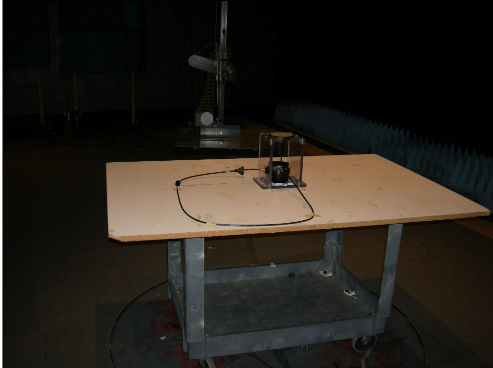
Figure 6: Radiated Emissions
