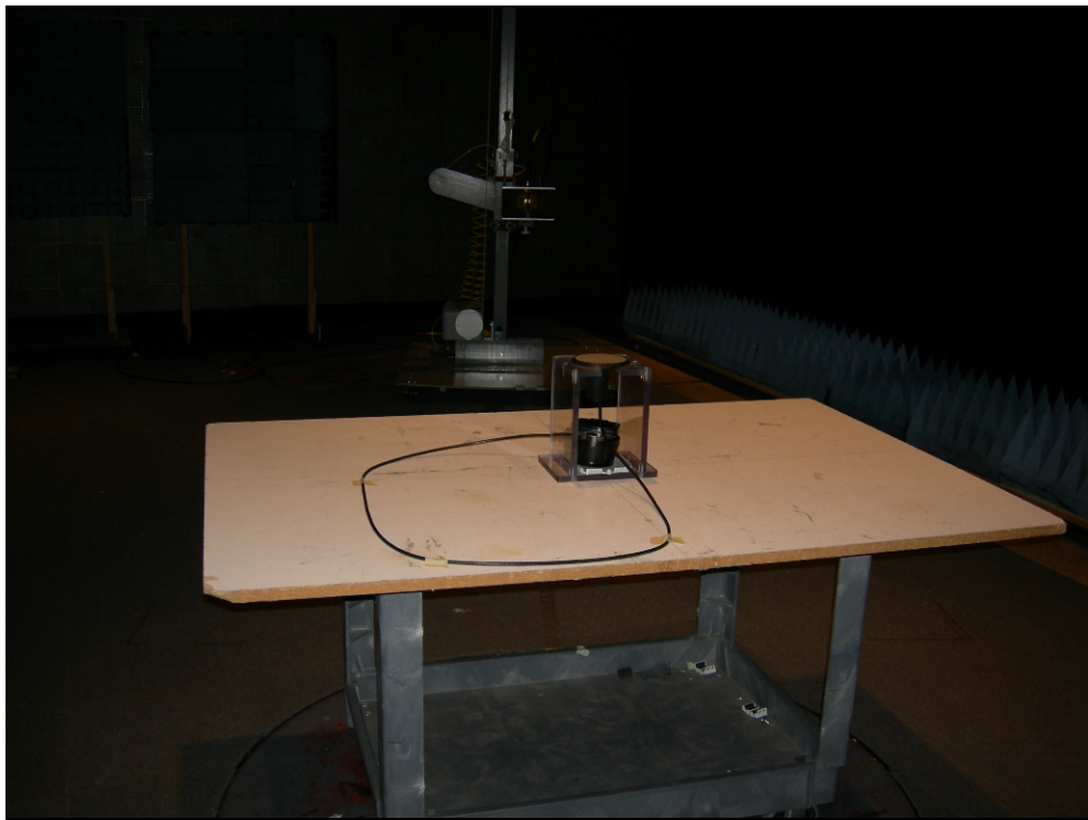
Figure 7: Radiated Emissions
