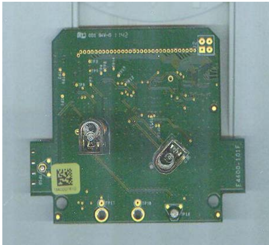
Figure 2: Internal Photo – PCB Bottom
