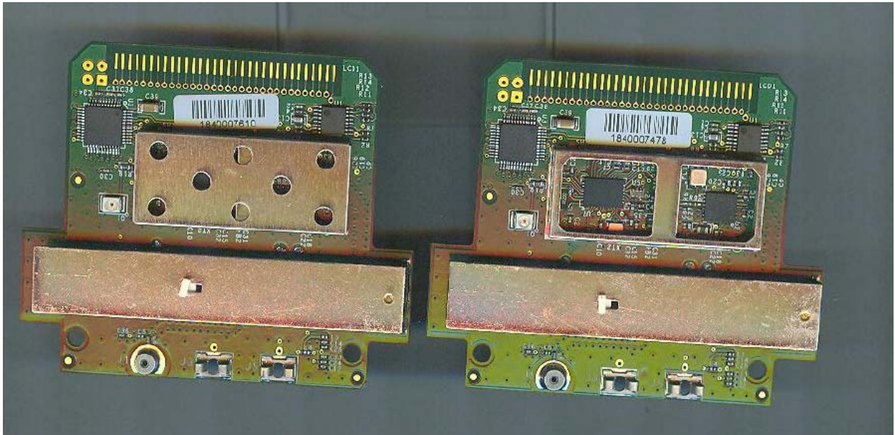
Figure 1: Internal Photo – PCB With (left) and without (right) Shield
