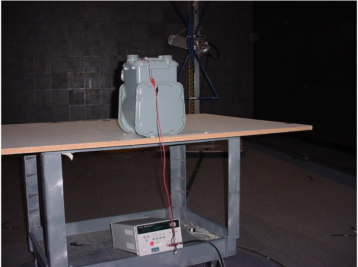
Figure 3: - Test Setup Photos – Radiated Emissions
