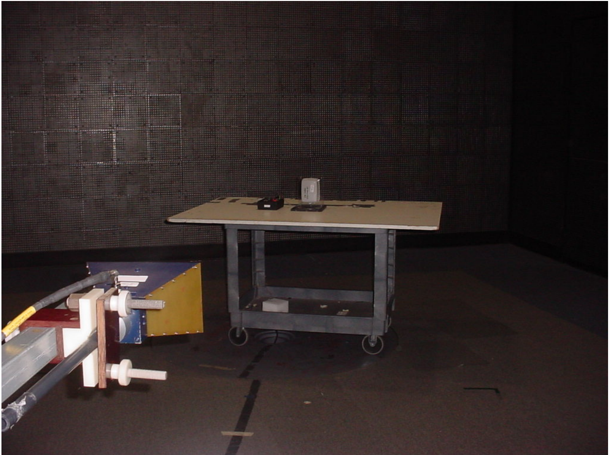
Figure 5: - Test Setup Photos – Spurious Emissions – Wall Mount Dipole Antenna
