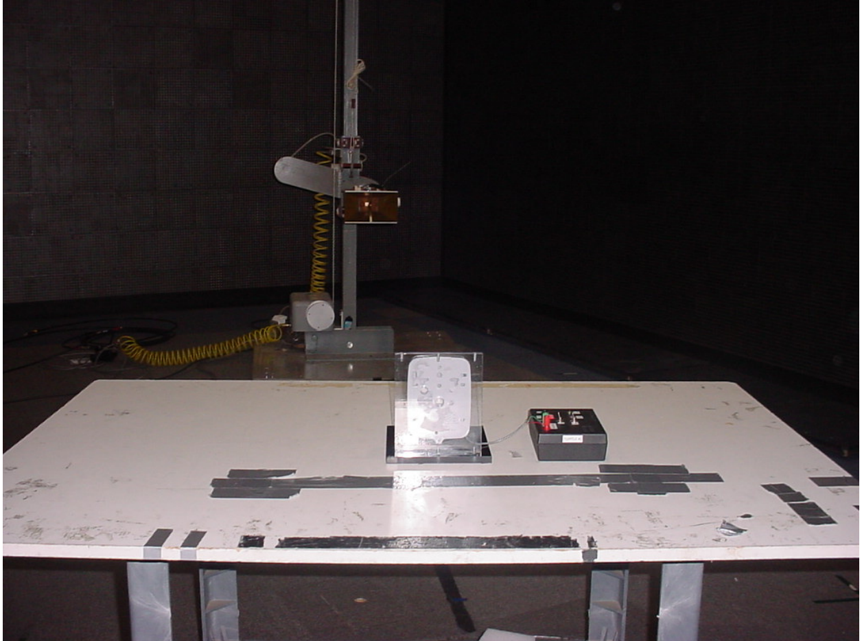
Figure 6: - Test Setup Photos – Spurious Emissions – Wall Mount Dipole Antenna
