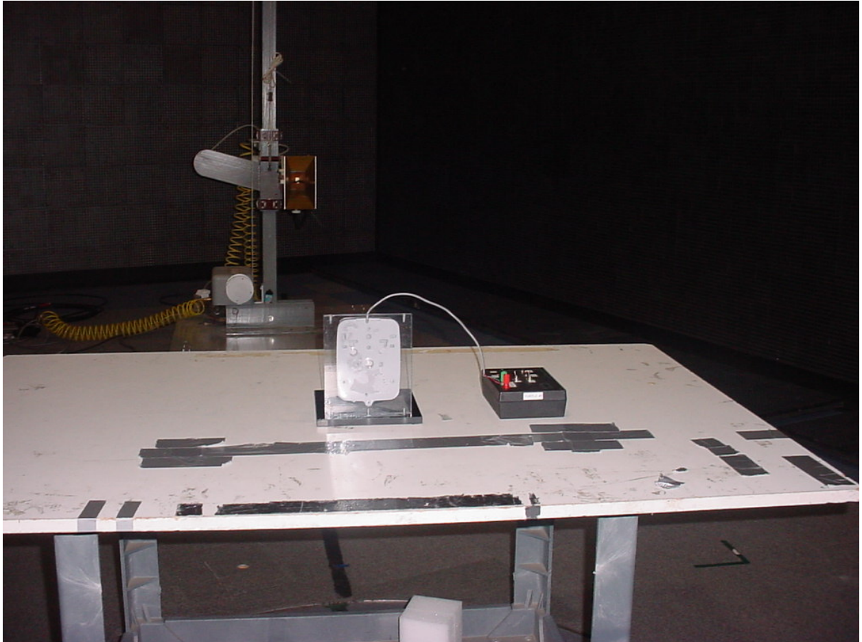
Figure 4: - Test Setup Photos – Spurious Emissions – Wall Mount PCB Antenna
