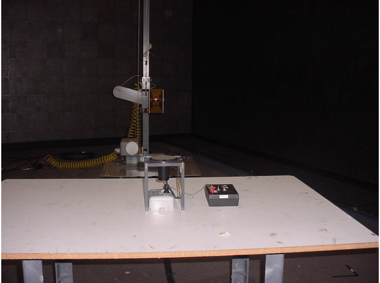
Figure 2: - Test Setup Photos – Spurious Emissions – Pit Mount Patch Antenna
