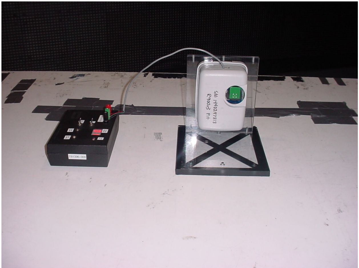
Figure 3: - Test Setup Photos – Spurious Emissions – Wall Mount PCB Antenna
