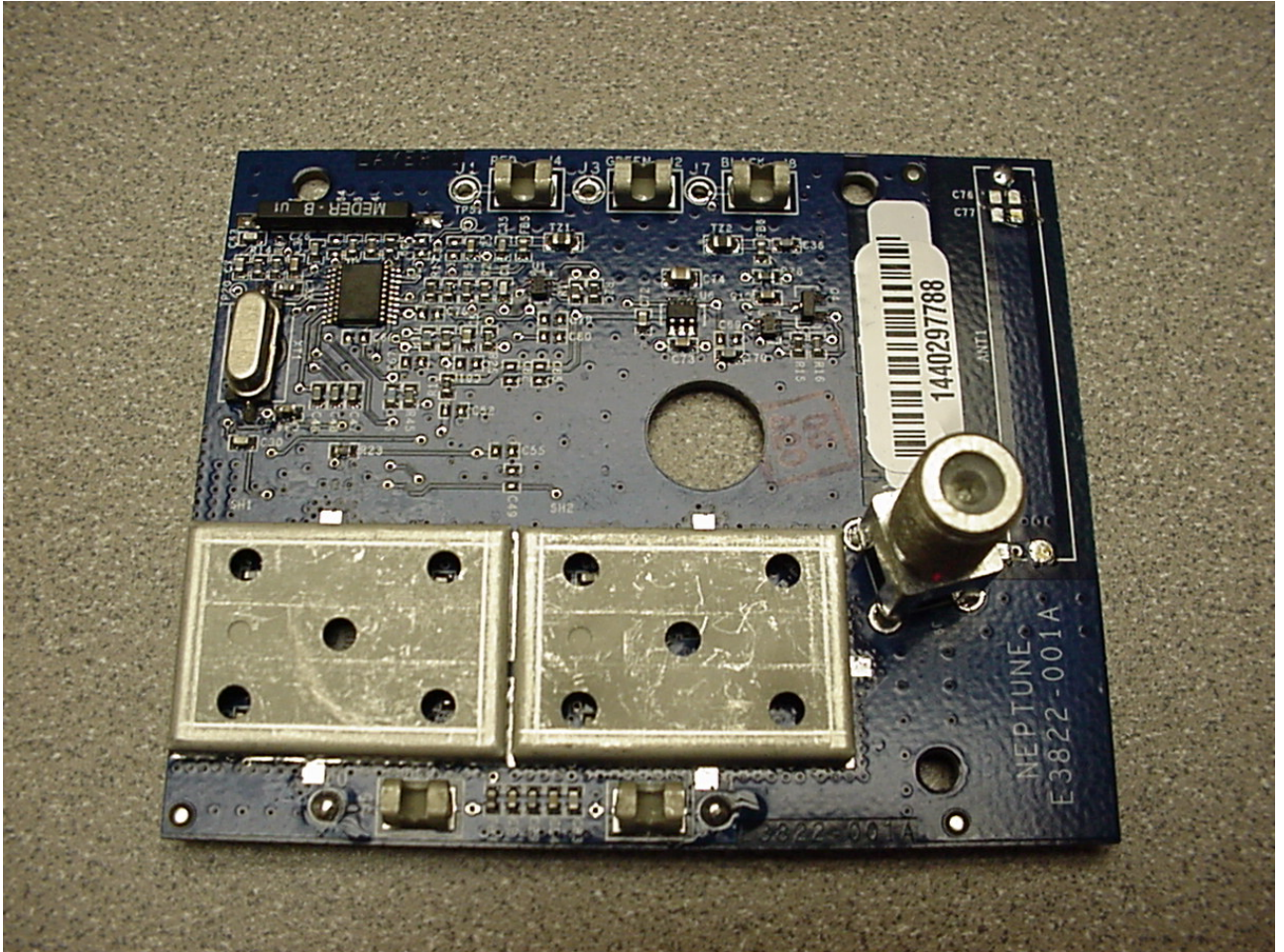
Figure 1: - Pit Mount / Wall Mount (External Antenna Connector) – Top View with Shields
