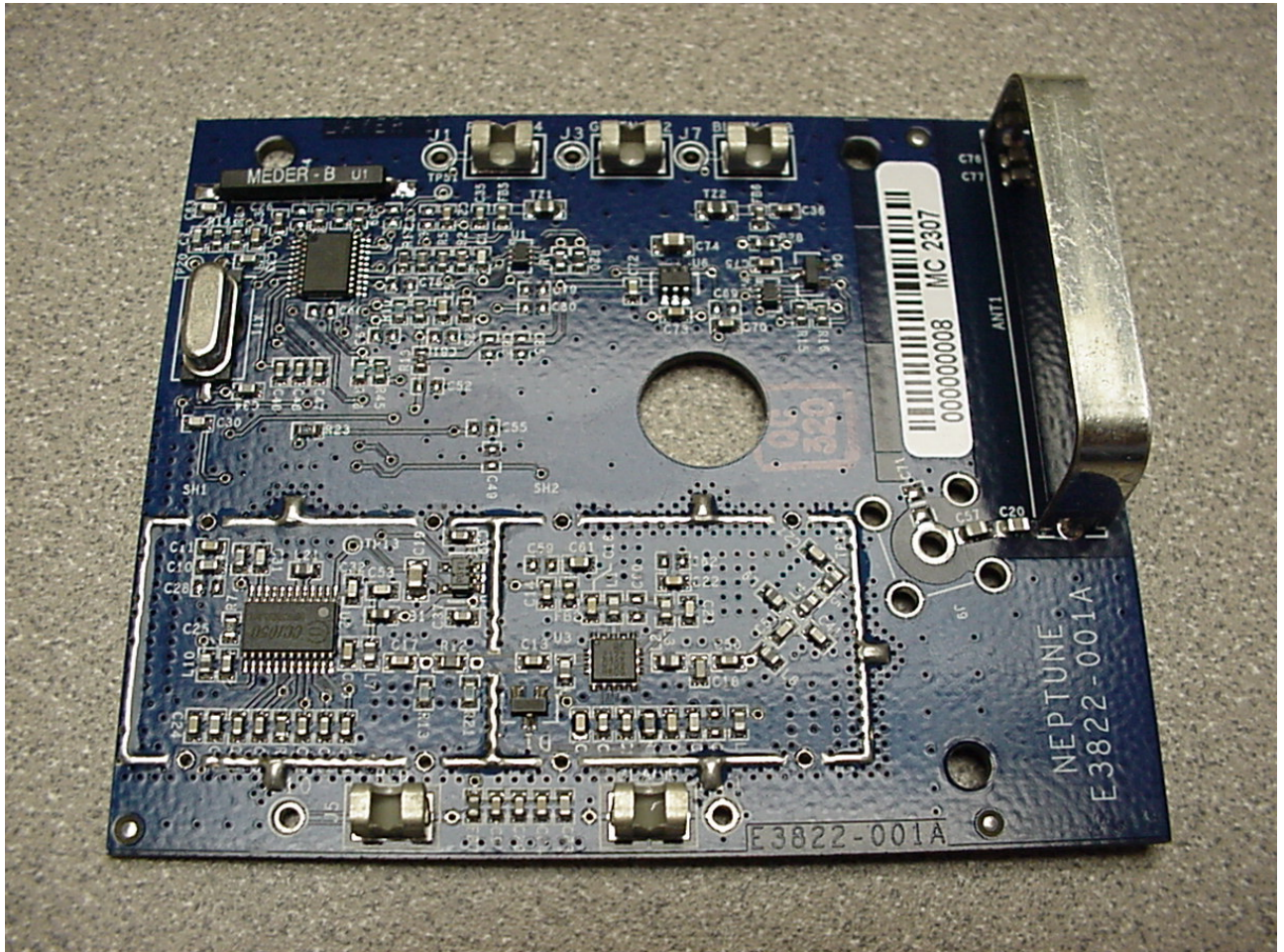
Figure 5: Wall Mount (Integral Antenna) – Top View without Shields
