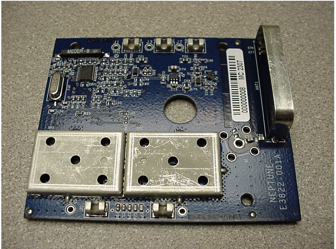
Figure 4: Wall Mount (Integral Antenna) – Top View with Shields
