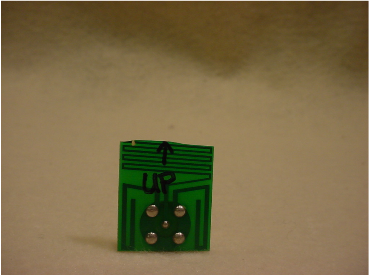
Figure 7: Wall Mount PCB Antenna - Front
