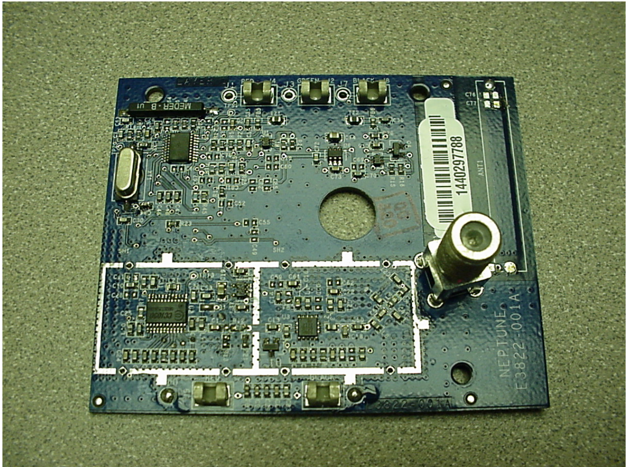
Figure 2: - Pit Mount / Wall Mount (External Antenna Connector) – Top View without Shields
