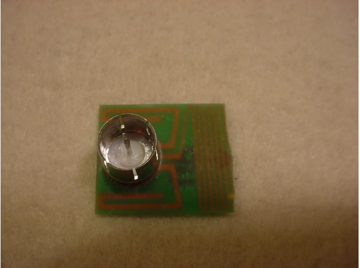
Figure 8: Wall Mount PCB Antenna - Back
