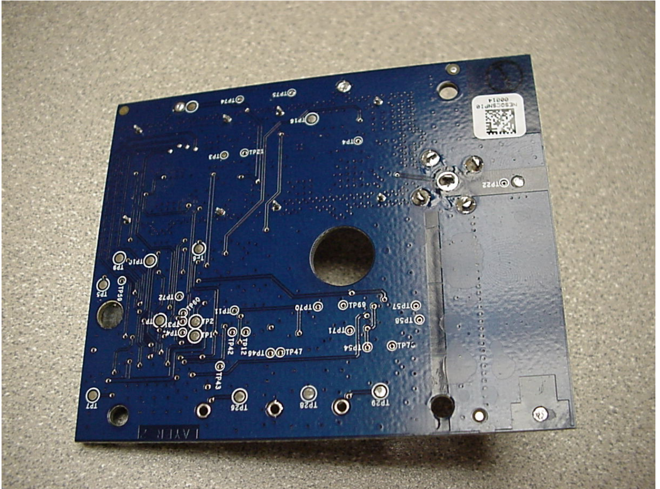
Figure 3: - Pit Mount / Wall Mount (External Antenna Connector) – Bottom View
