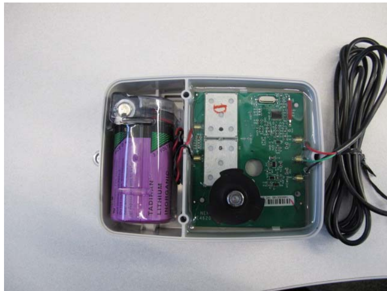
Figure 1: Internal View
