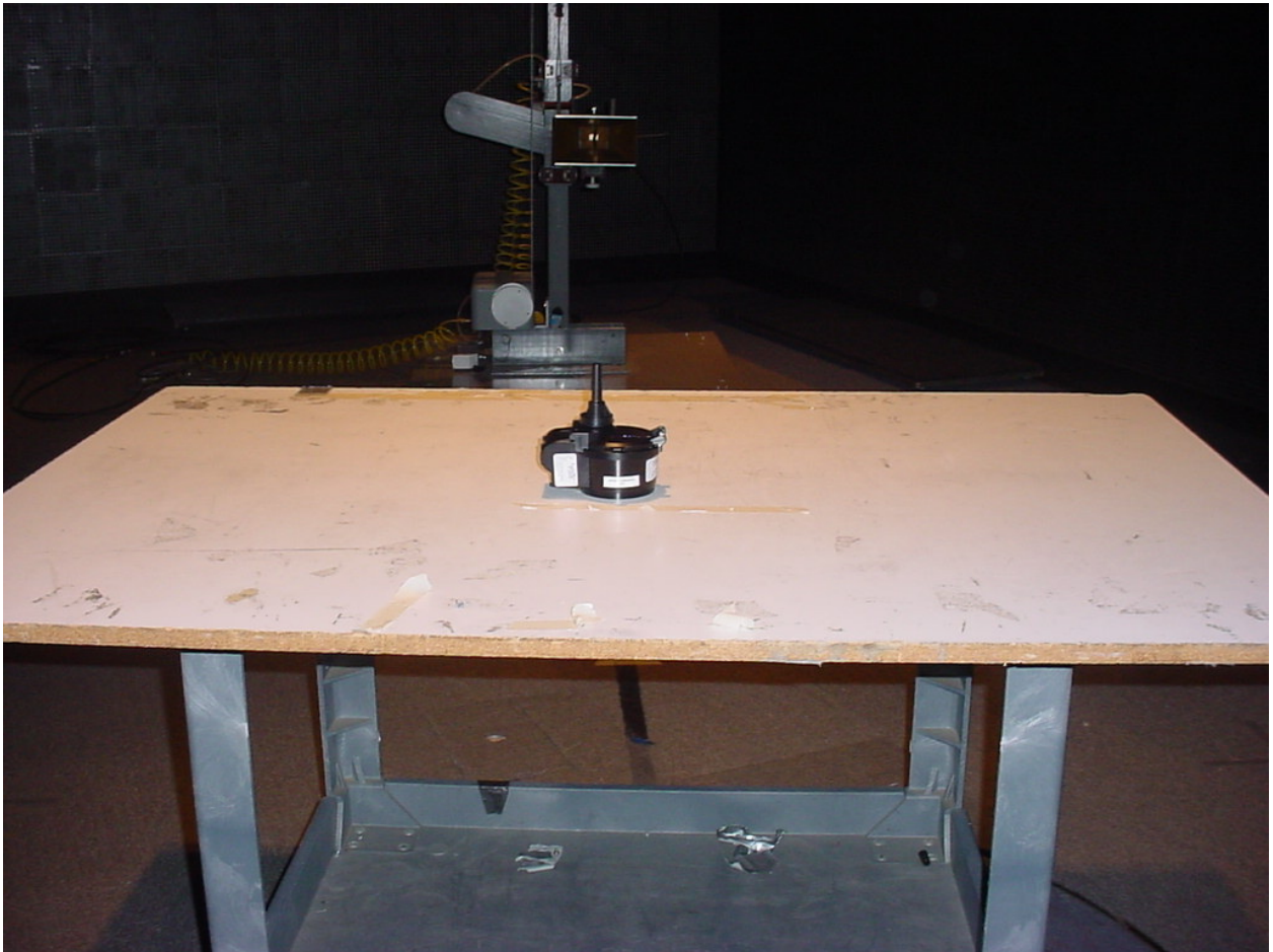
Figure 2: Test Setup – Radiated Emissions – Pit Monopole Antenna
