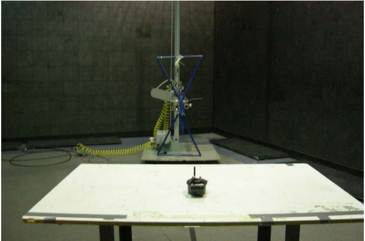
Figure 6: Test Setup – Radiated Emissions – Unintentional Pit Monopole Configuration
