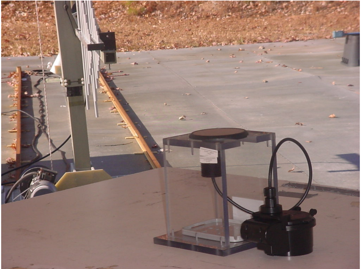
Figure 2: Test Setup – Radiated Emissions – Intentional Pit Patch Configuration
