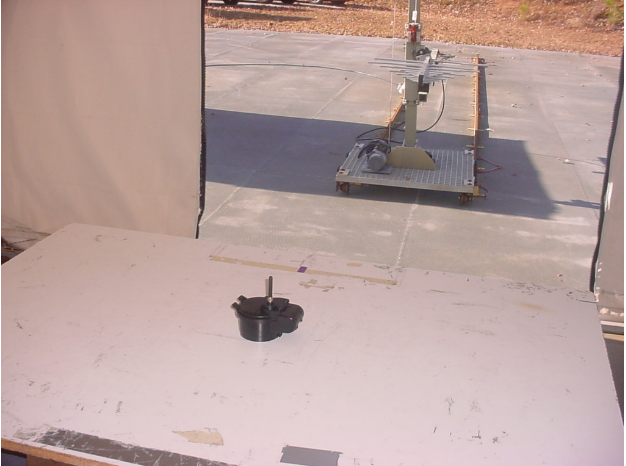
Figure 3: Test Setup – Radiated Emissions – Intentional Pit Monopole Configuration
