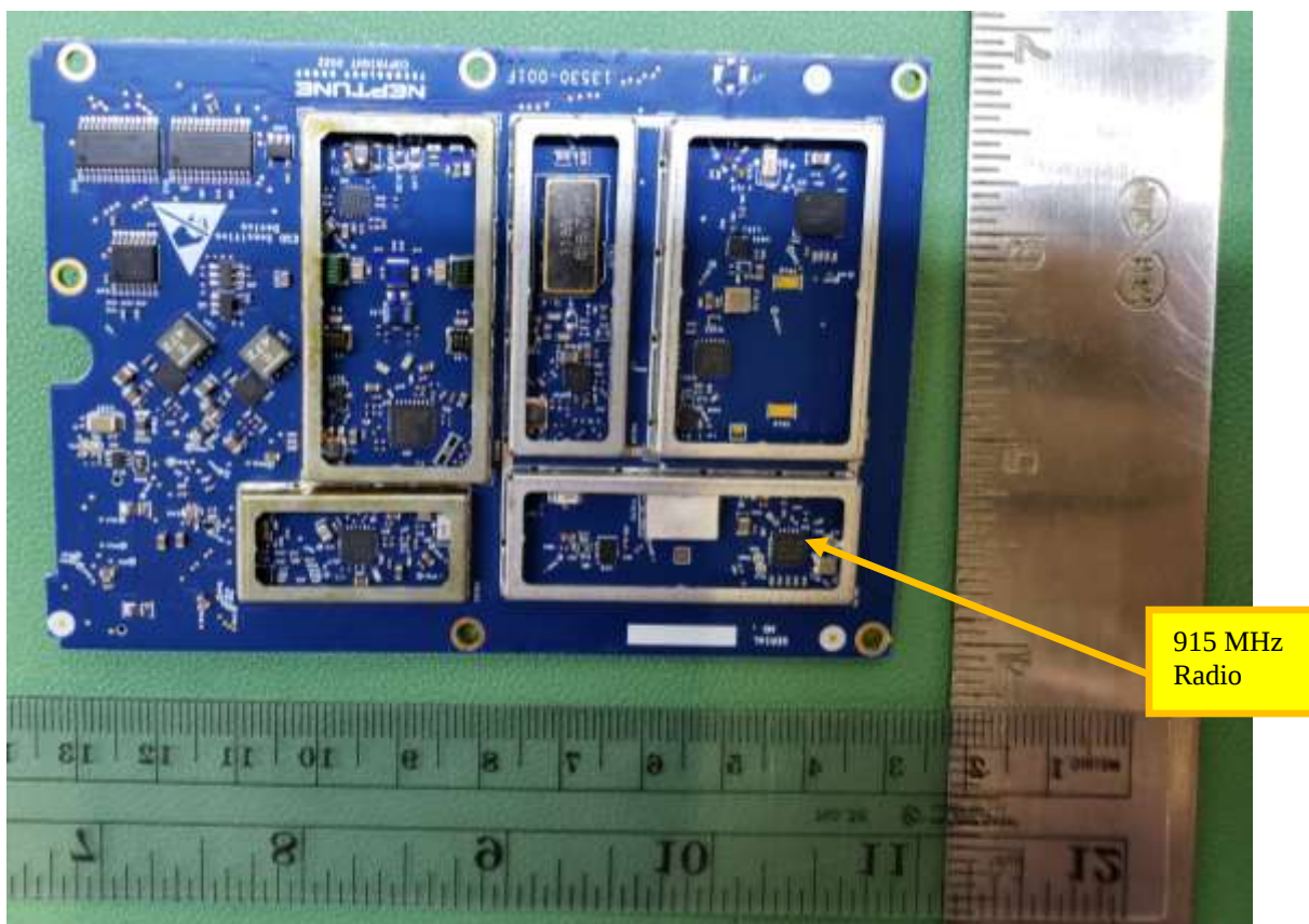
Figure 6. Radio, Shield Removed (Customer Radio Section)
