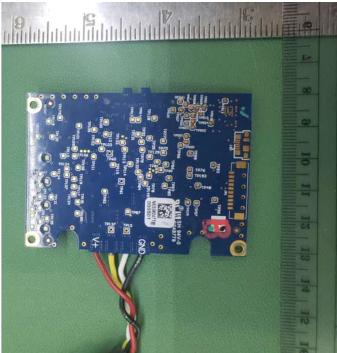
Figure 8. Control Electronics PCB 1 Bottom
