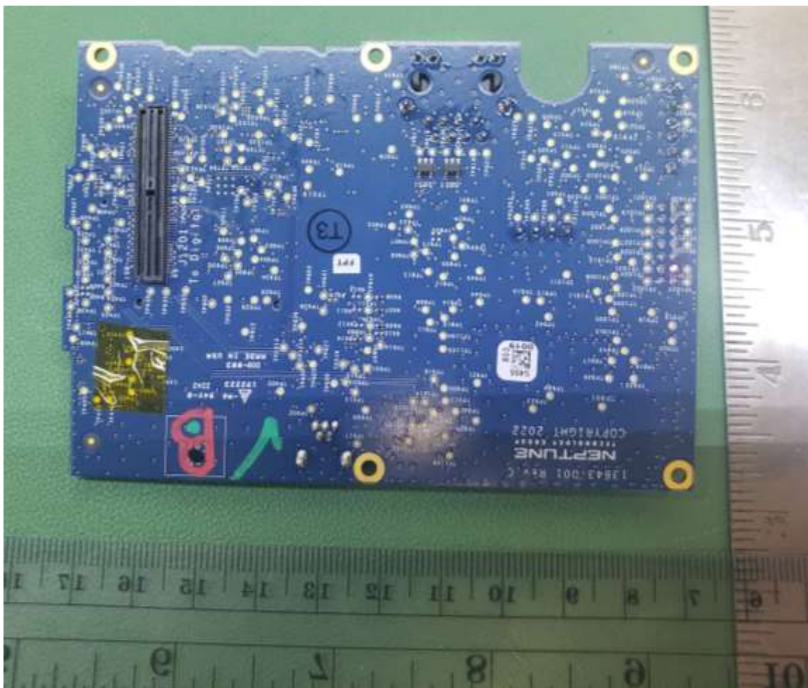
Figure 10. Control Electronics PCB 2 Bottom
