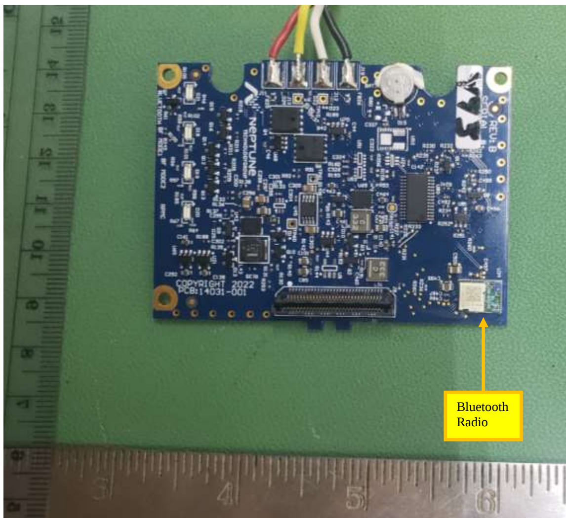
Figure 7. Control Electronics PCB 1 Top
