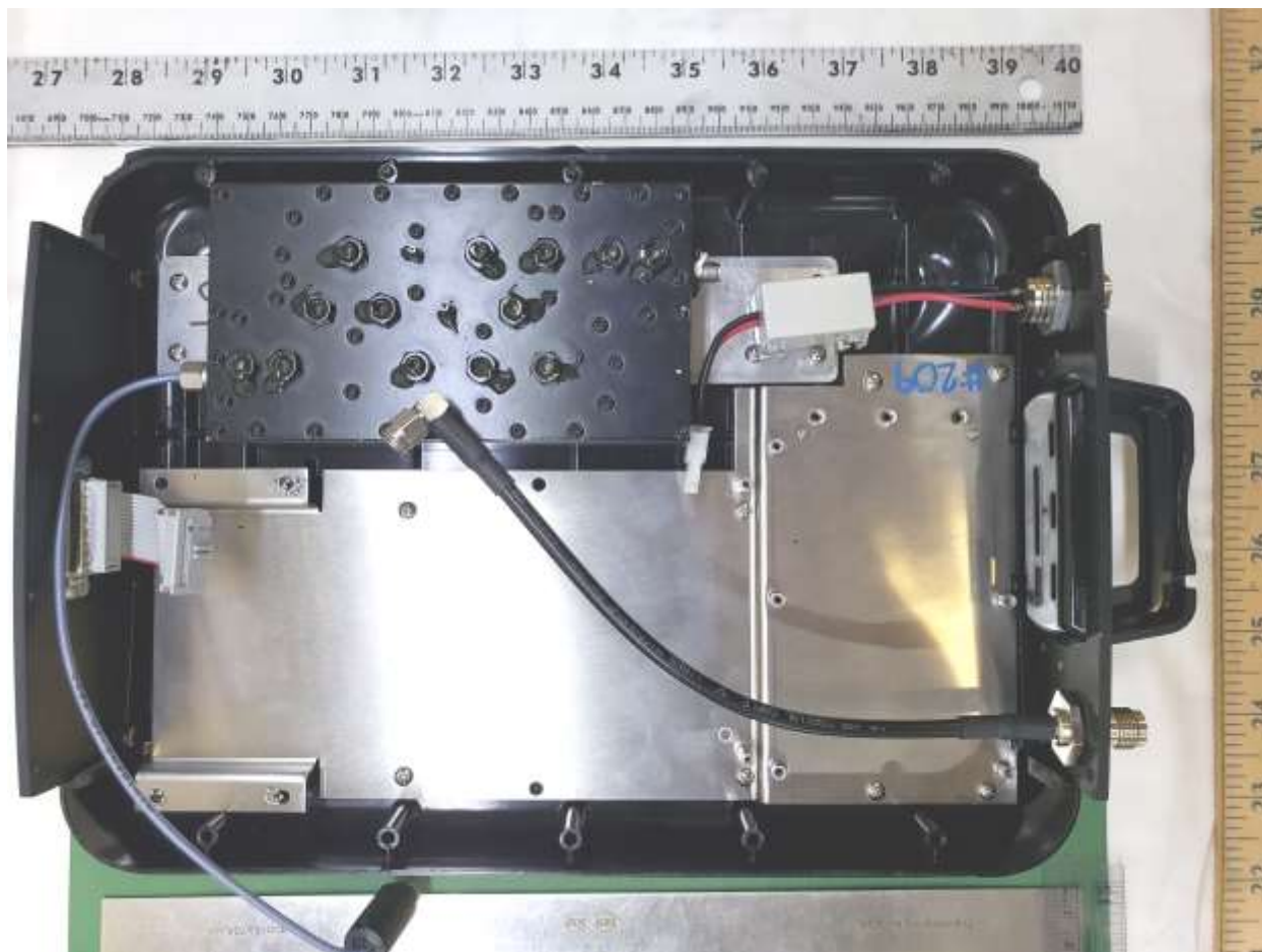
Figure 3. Enclosure, Electronics Removed
