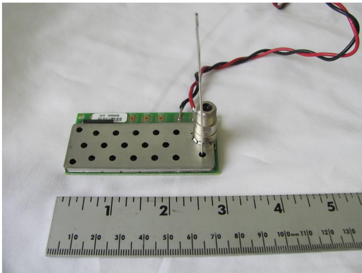
Figure 4. Internal Antenna Installed in Module
