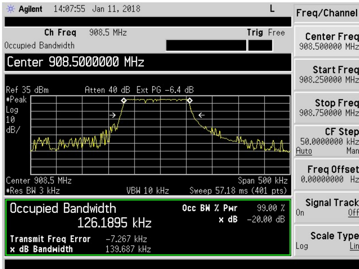
Figure 17. Twenty dB Bandwidth – Mid Channel
