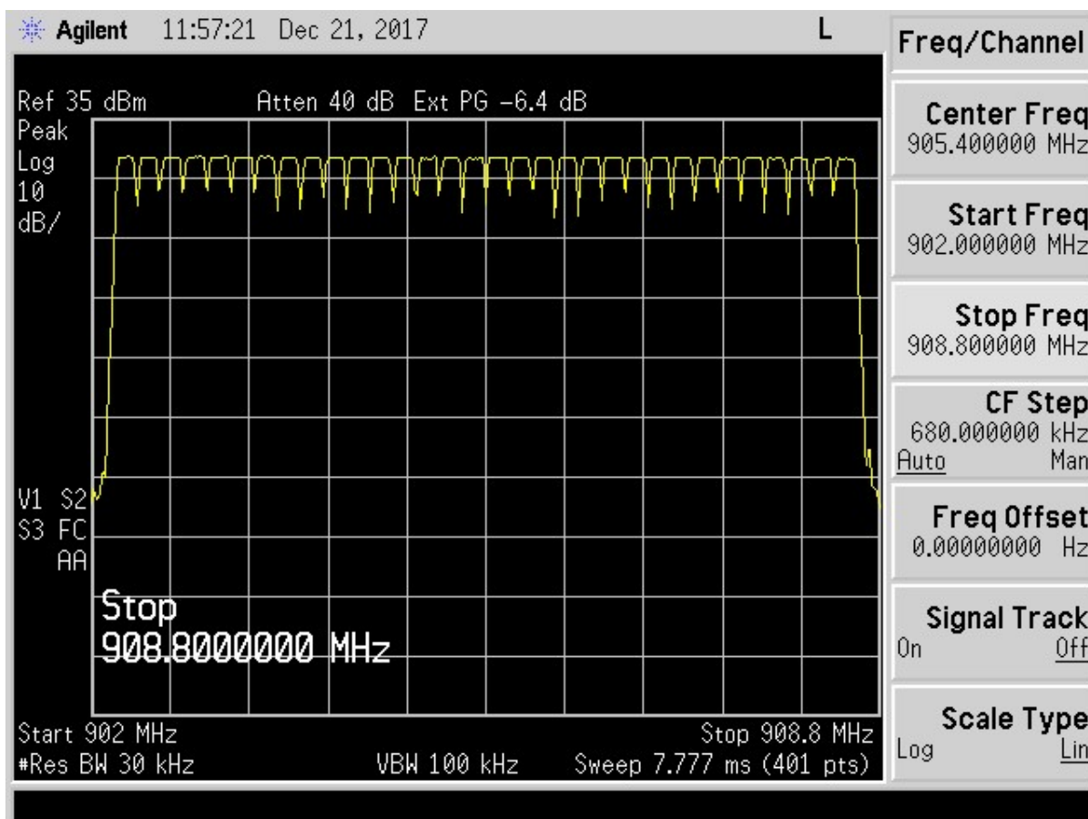
Figure 22. Hopping Channels 1 through 32
