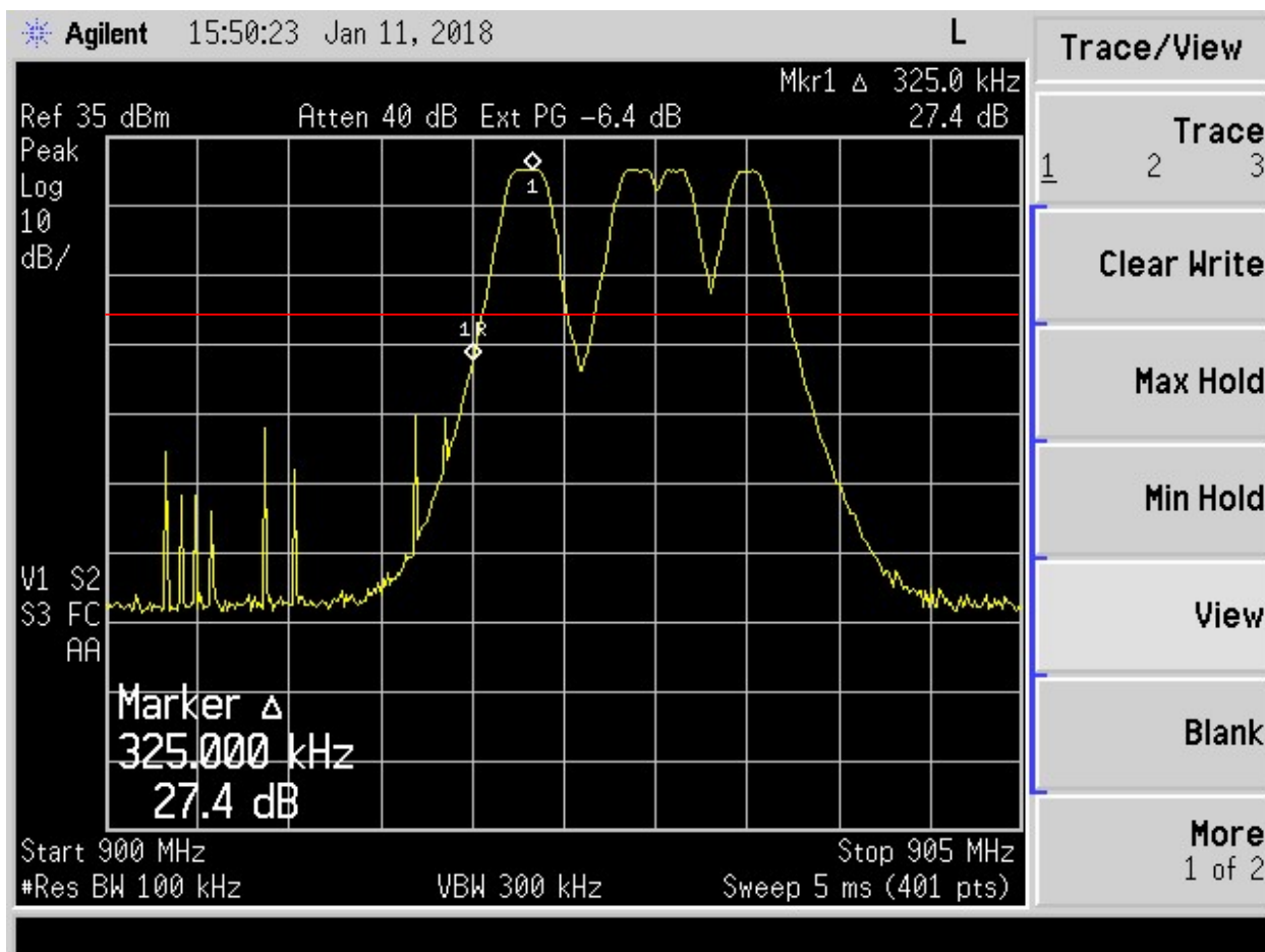
Figure 14. Band Edge Compliance, Low Channel Delta – Channel Hopping FHSS Modulation (Conducted)
