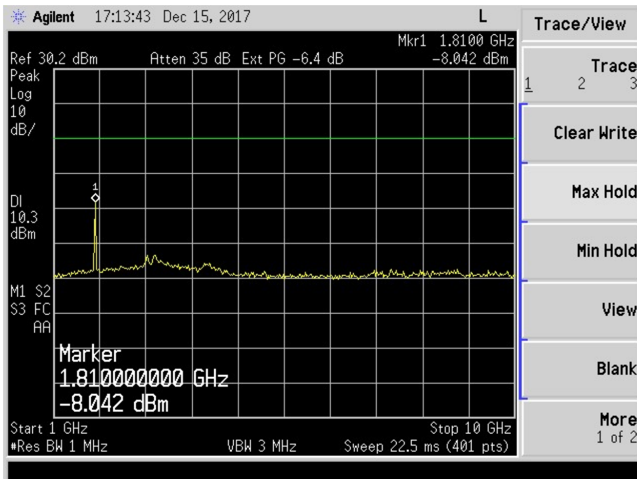
Figure 3. Antenna Conducted Emissions Low, 1 to 10 GHz
