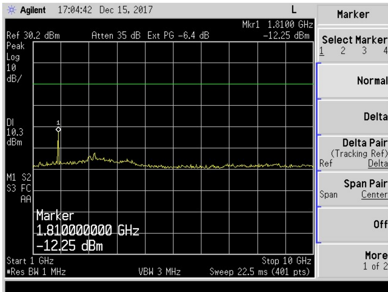
Figure 5. Antenna Conducted Emissions Mid, 1 to 10 GHz
