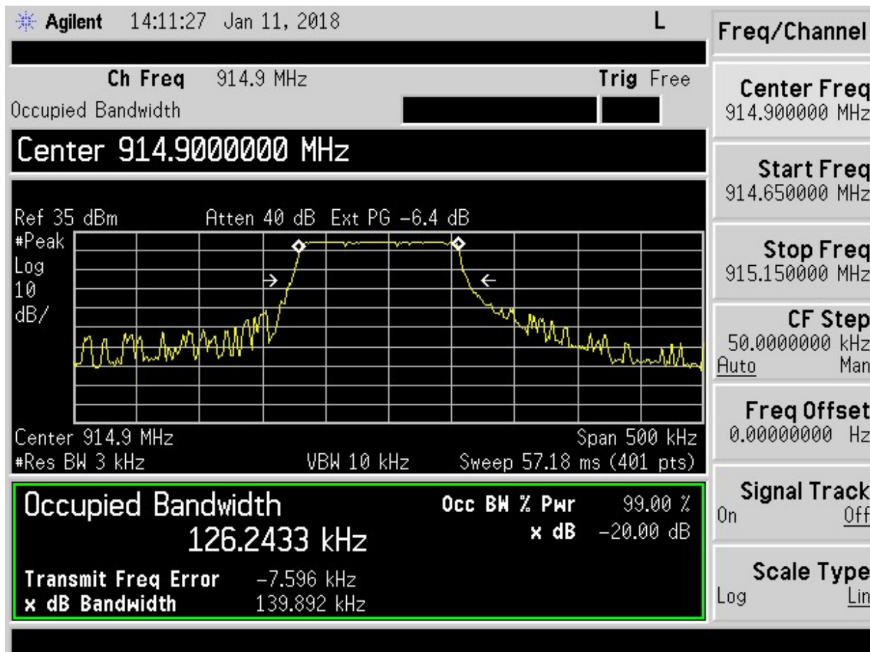
Figure 18. Twenty dB Bandwidth – High Channel
