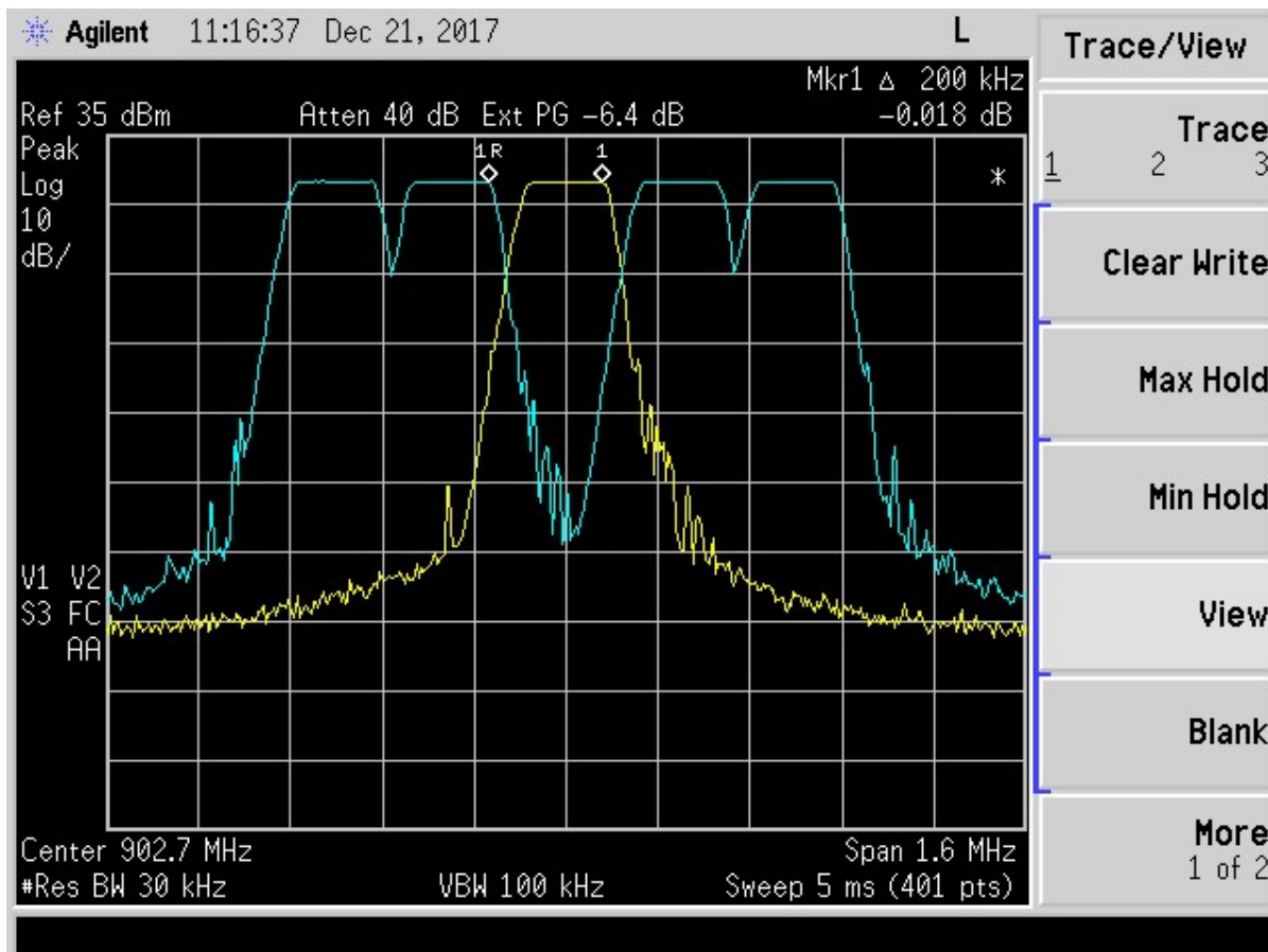
Figure 24. Channel Separation
