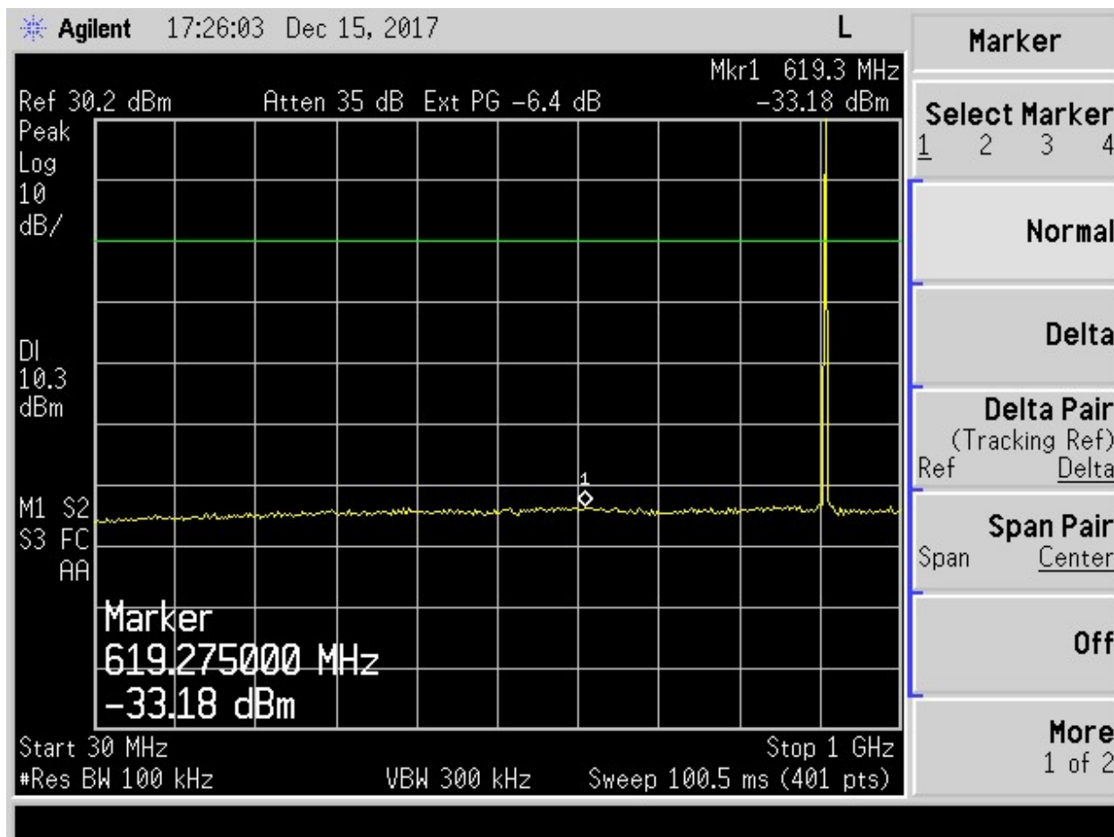
Figure 4. Antenna Conducted Emissions Mid, 30 MHz to 1 GHz
