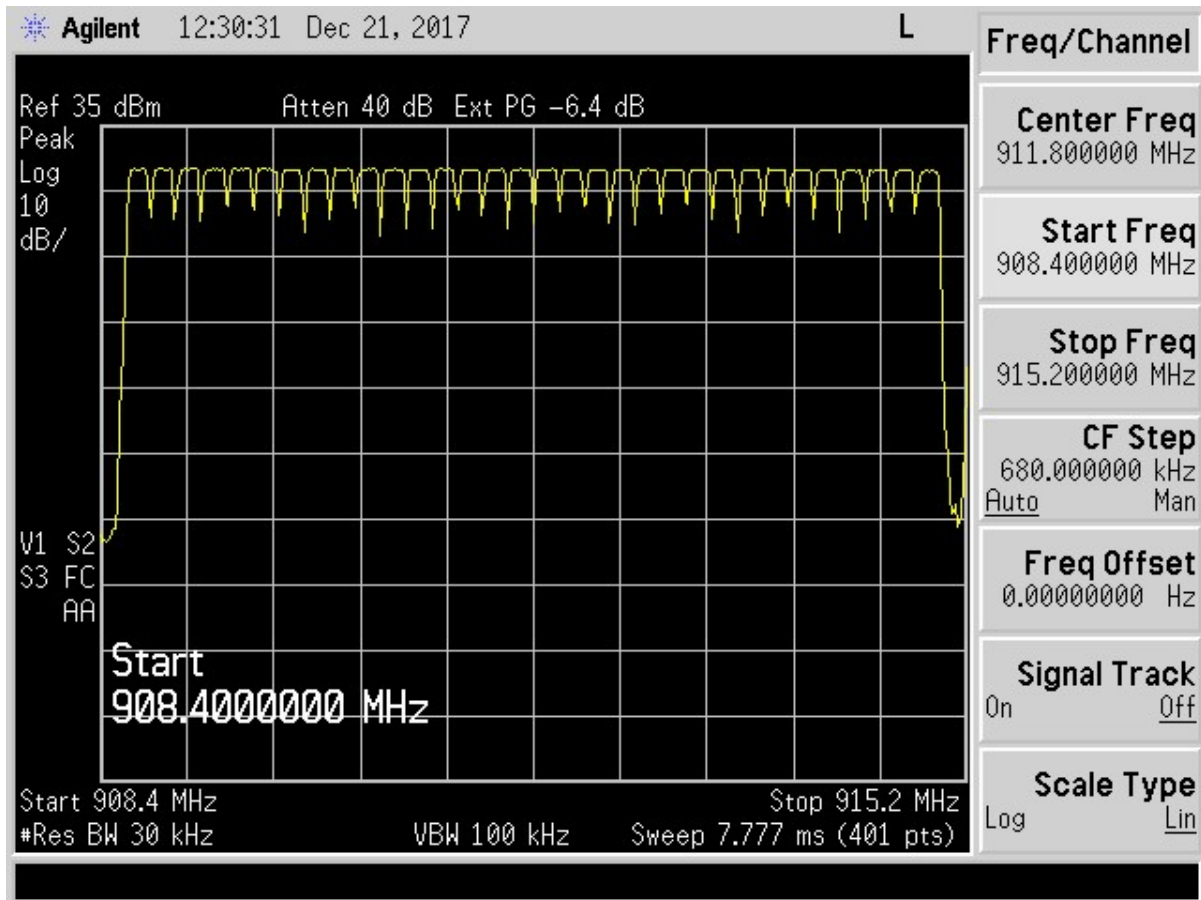
Figure 23. Hopping Channels 33 - 64
