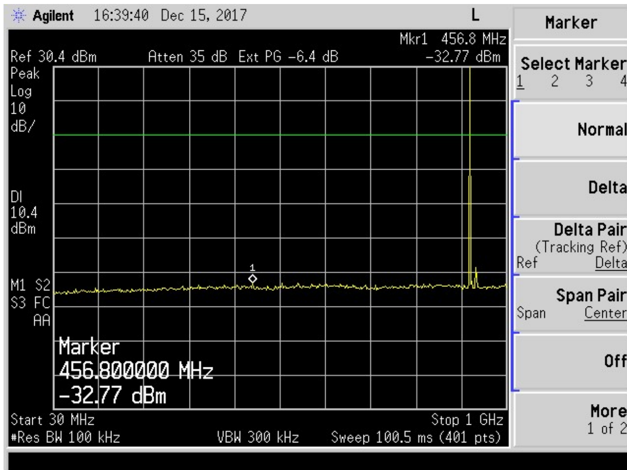
Figure 6. Antenna Conducted Emissions High, 30 MHz to 1 GHz
