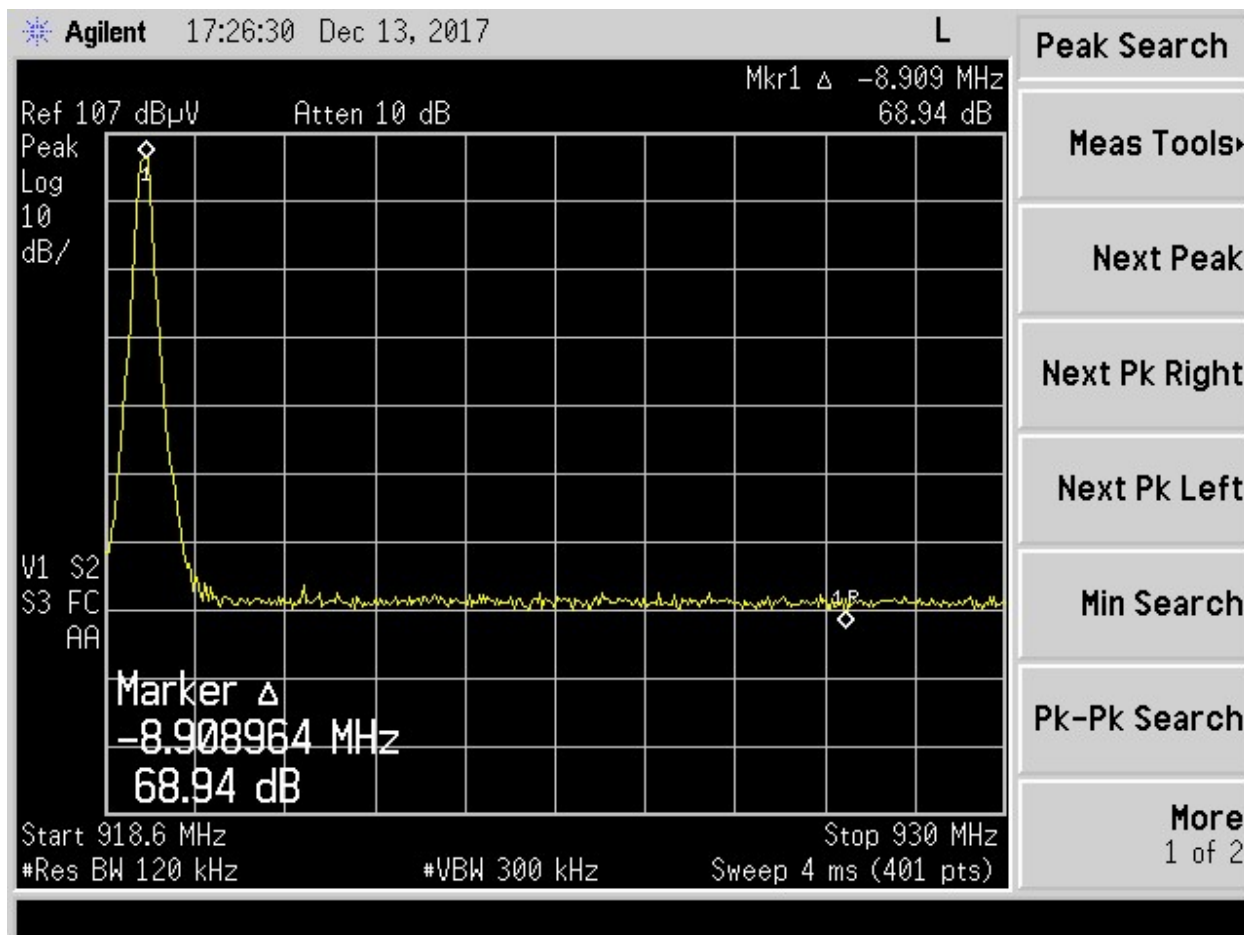
Figure 11. Band Edge Compliance, High Channel Delta – Antenna 2
