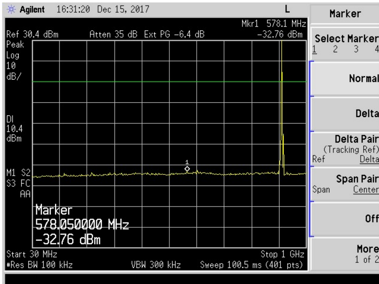
Figure 4. Antenna Conducted Emissions Low, 30 MHz to 1 GHz
