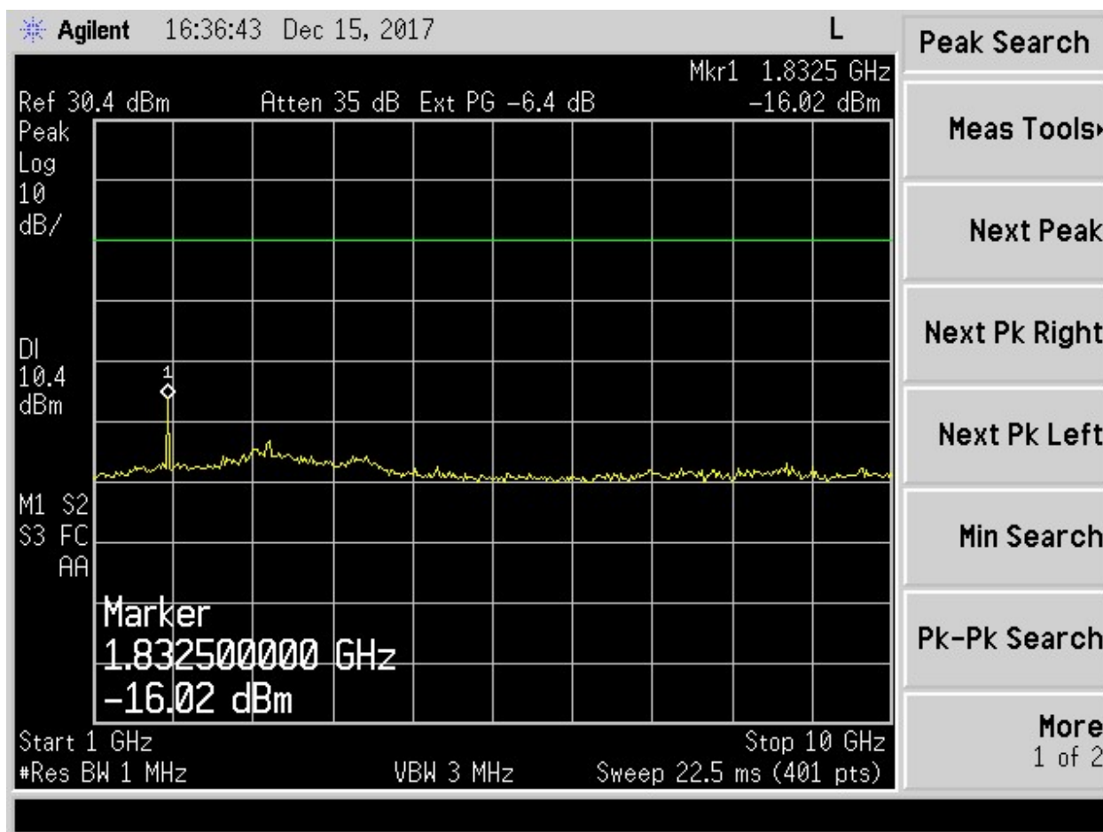
Figure 7. Antenna Conducted Emissions High, 1 to 10 GHz
