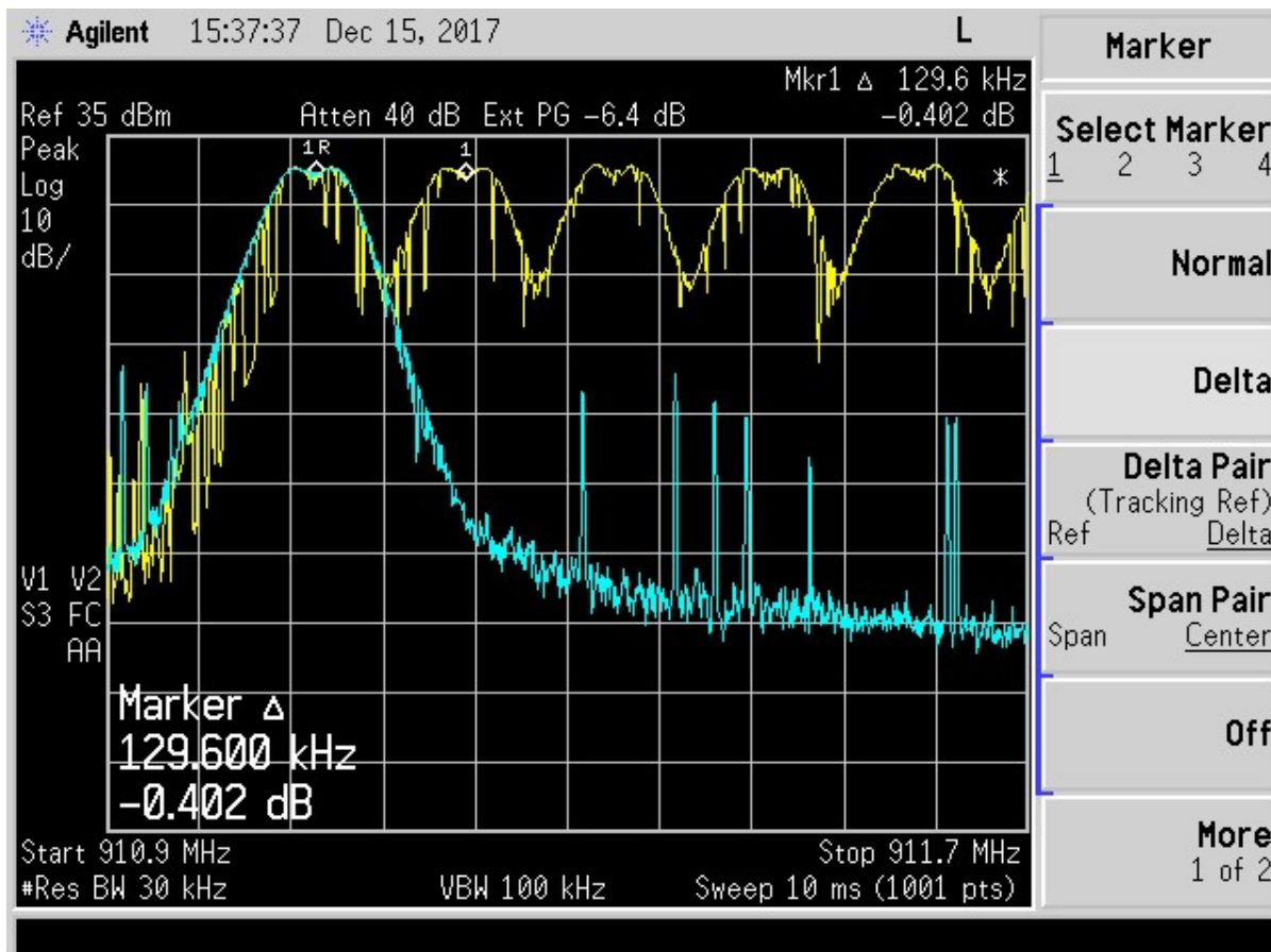
Figure 21. Channel Separation
