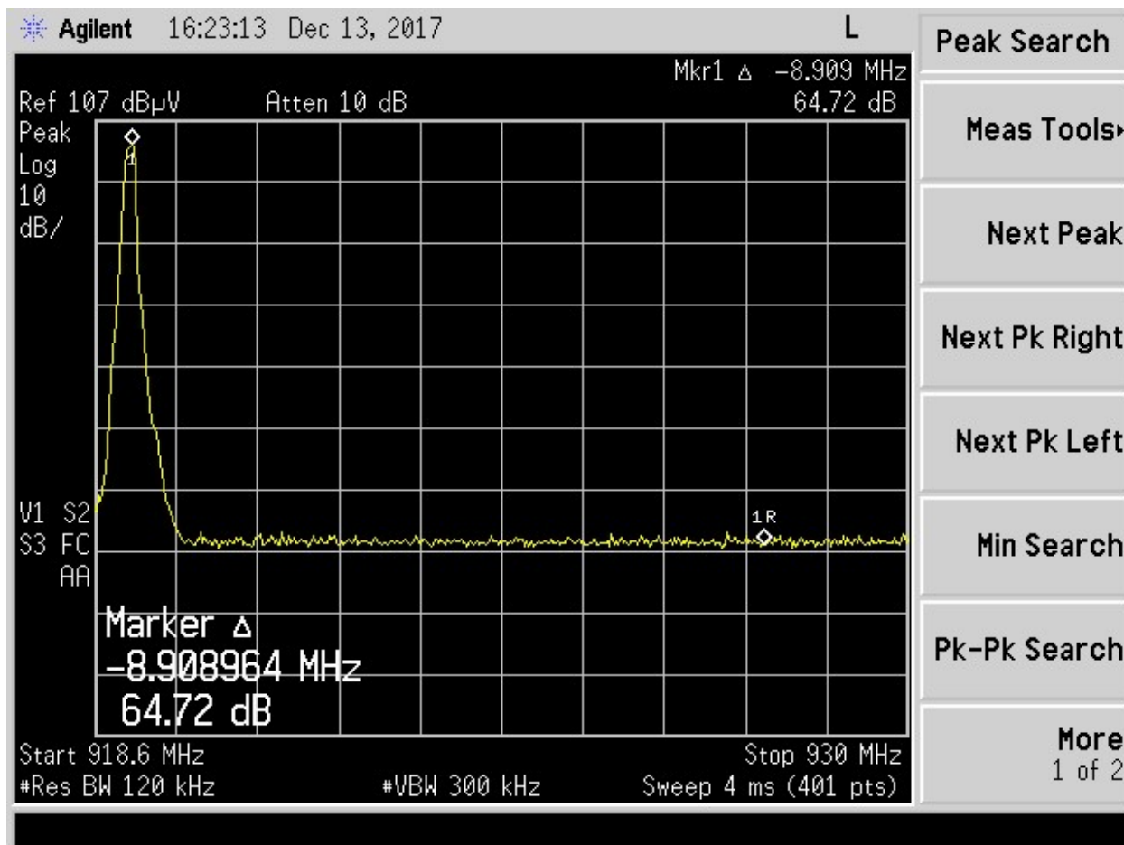
Figure 13. Band Edge Compliance, High Channel Delta – Antenna 3
