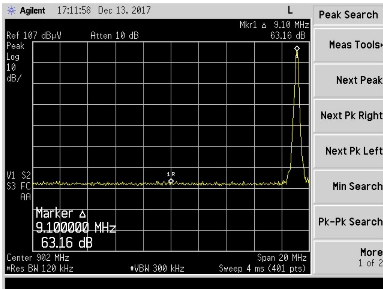
Figure 10. Band Edge Compliance, Low Channel Delta – Antenna 2
