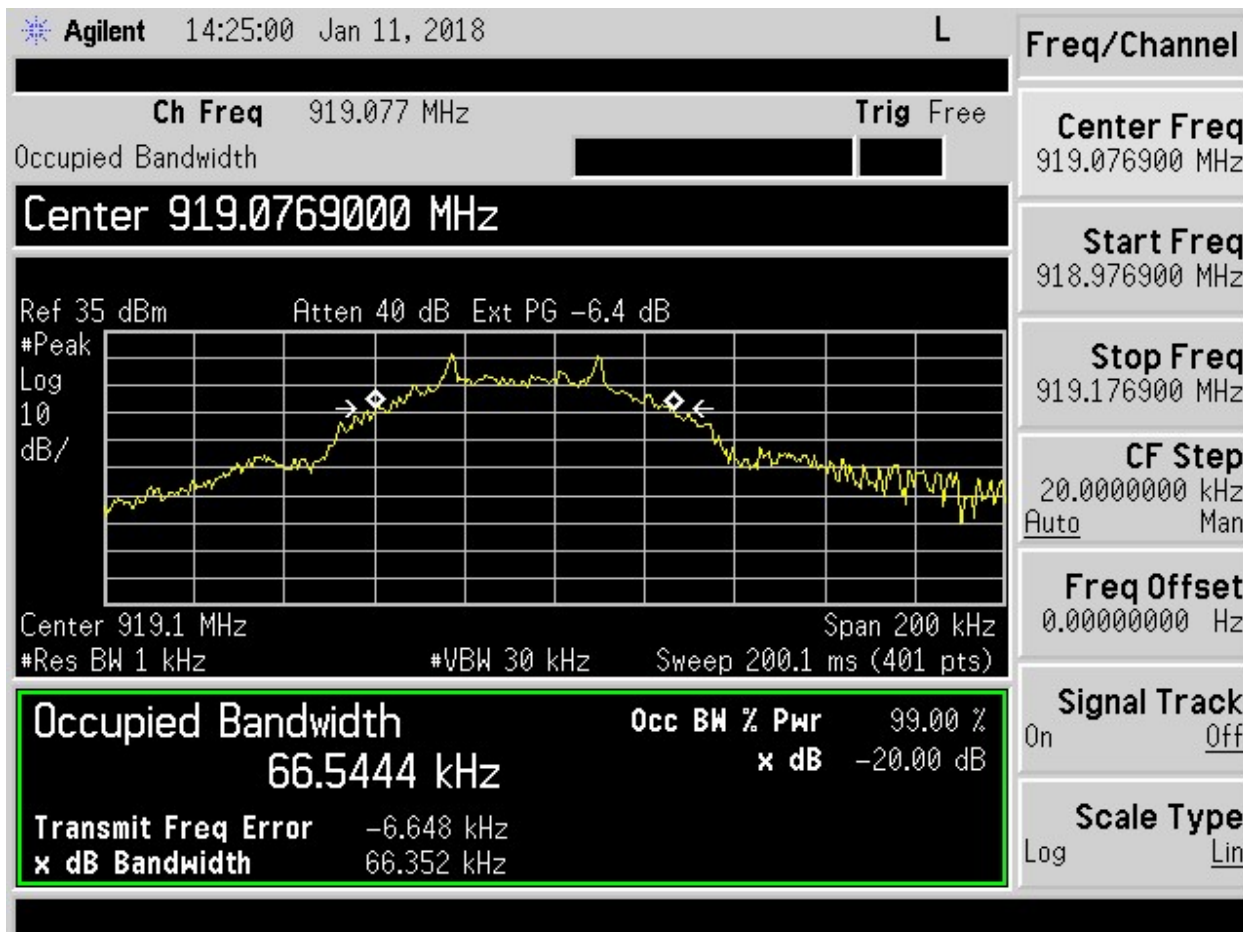
Figure 17. Twenty dB Bandwidth – High Channel
