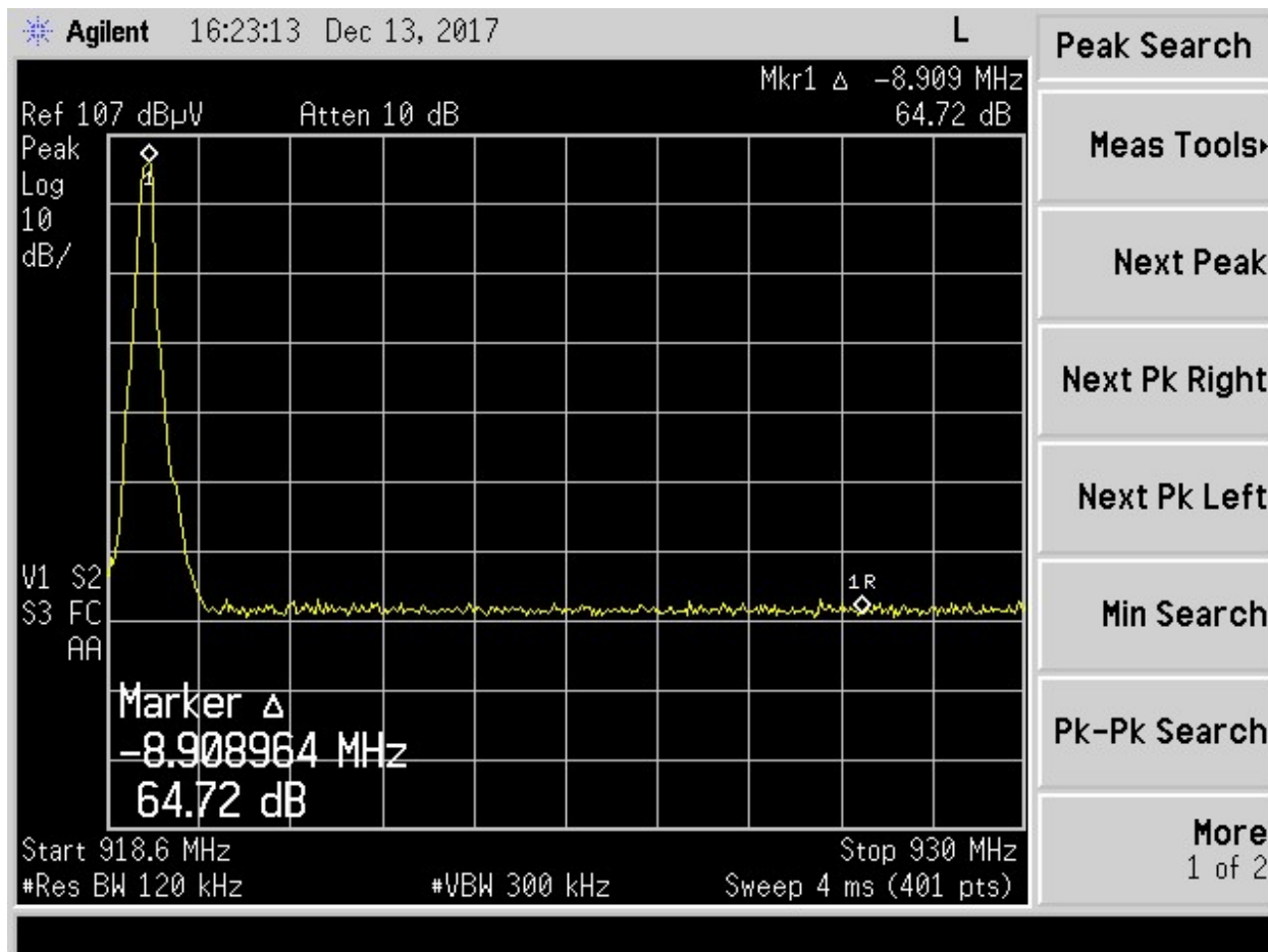
Figure 9. Band Edge Compliance, High Channel Delta – Antenna 1
