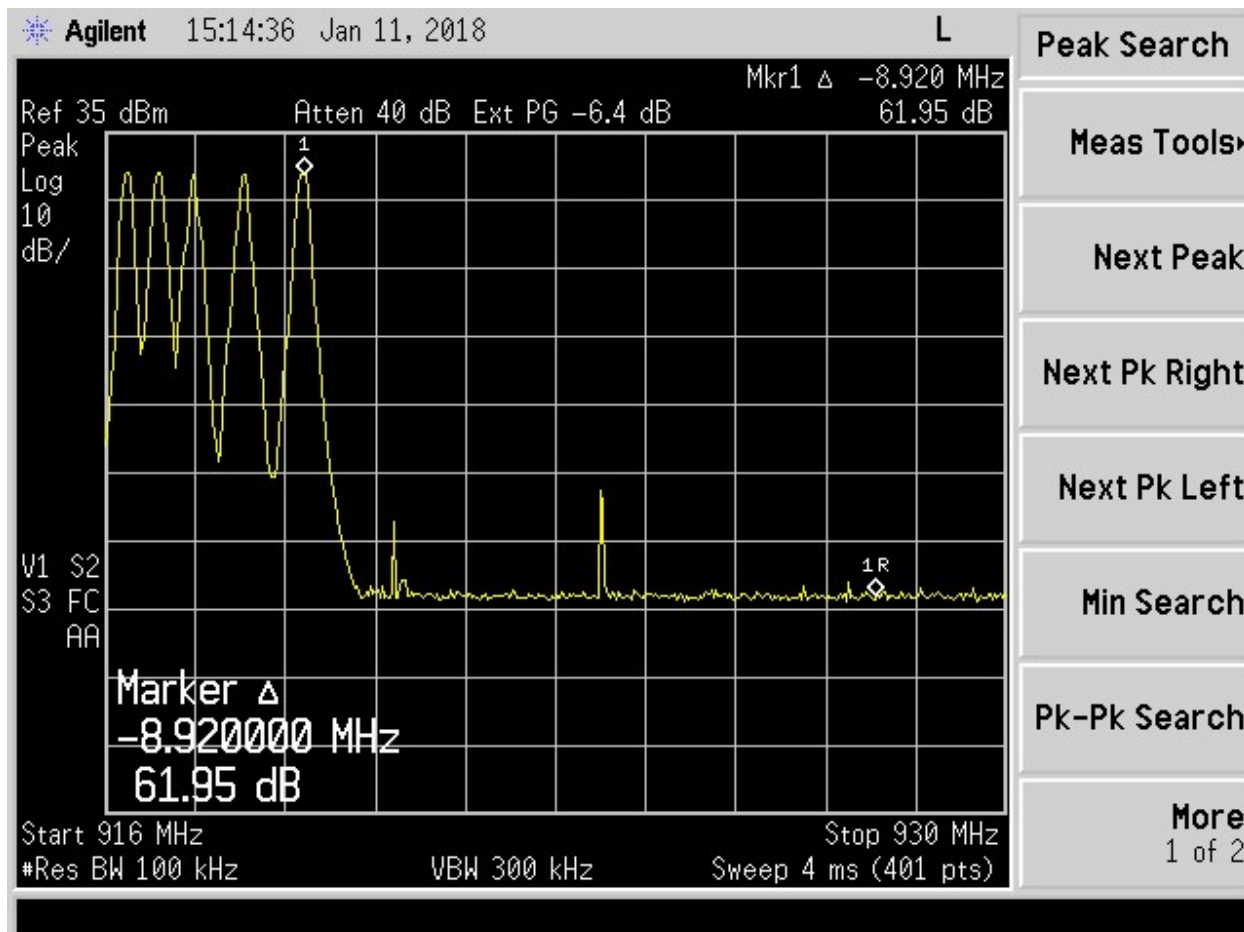
Figure 15. Band Edge Compliance, High Channel Delta – Channel Hopping GFSK Modulation (Conducted)
