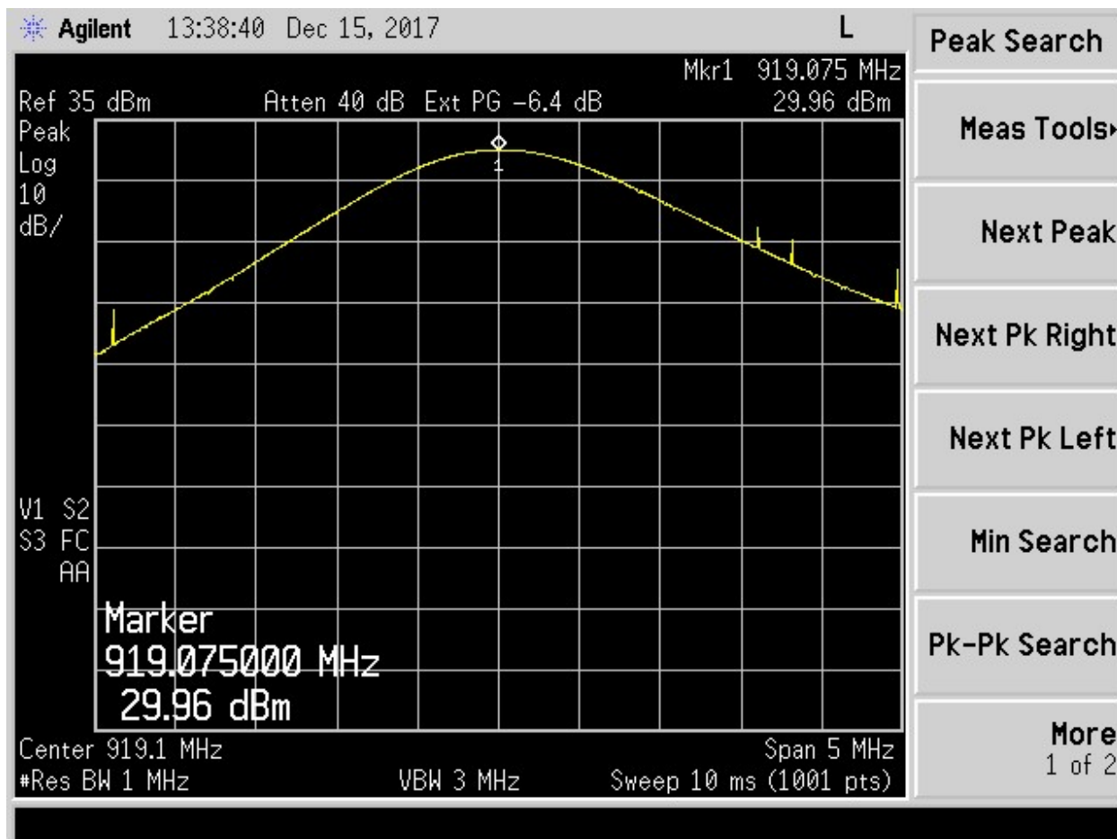
Figure 19. Peak Antenna Conducted Output Power, High Channel
