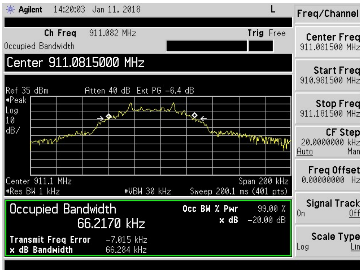
Figure 16. Twenty dB Bandwidth – Low Channel
