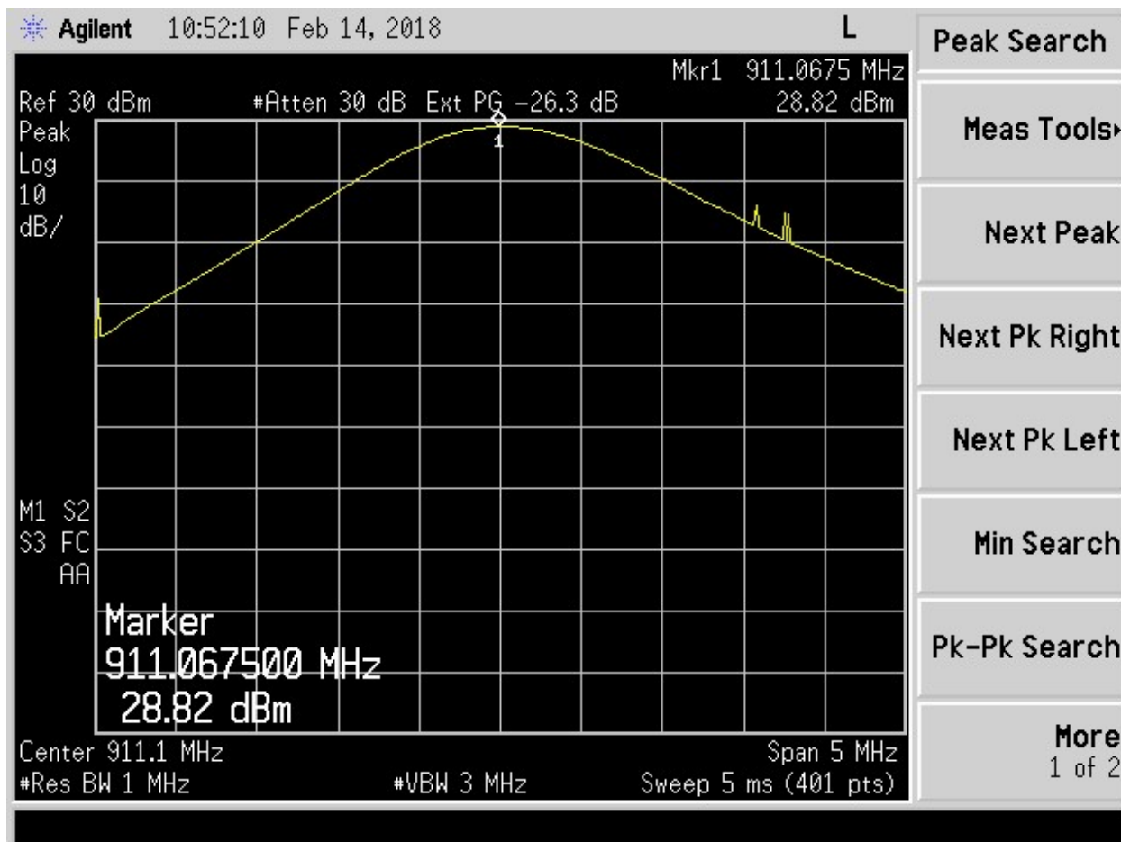
Figure 18. Peak Antenna Conducted Output Power, Low Channel
