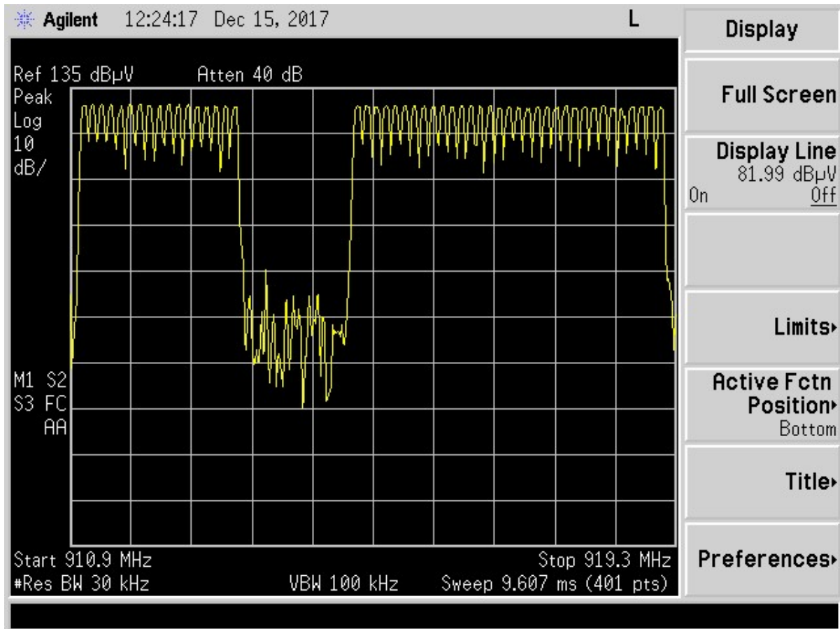
Figure 20. Hopping Channels 1 through 50
