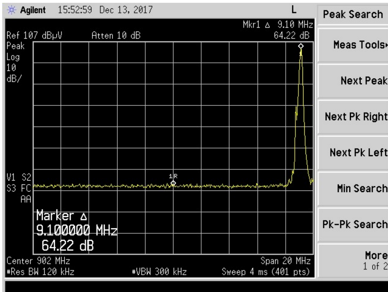
Figure 12. Band Edge Compliance, Low Channel Delta – Antenna 3
