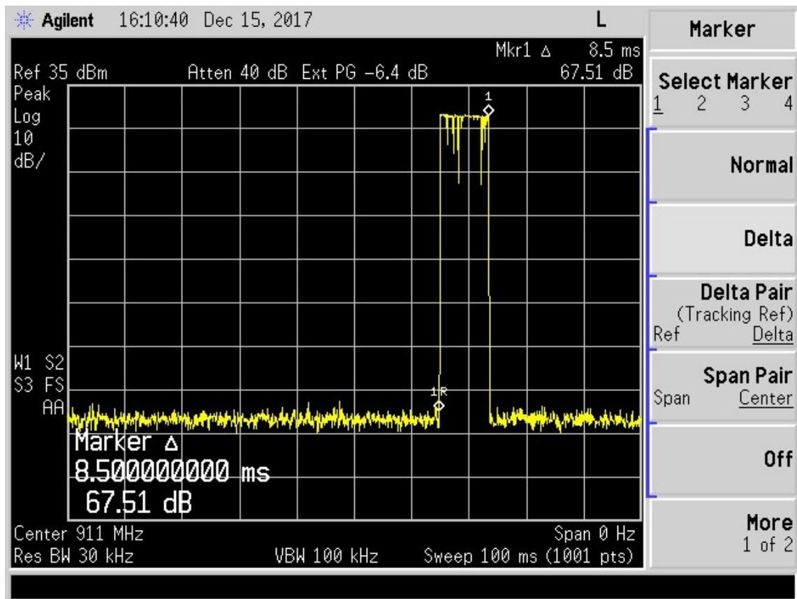
Figure 2. Pulse Width
