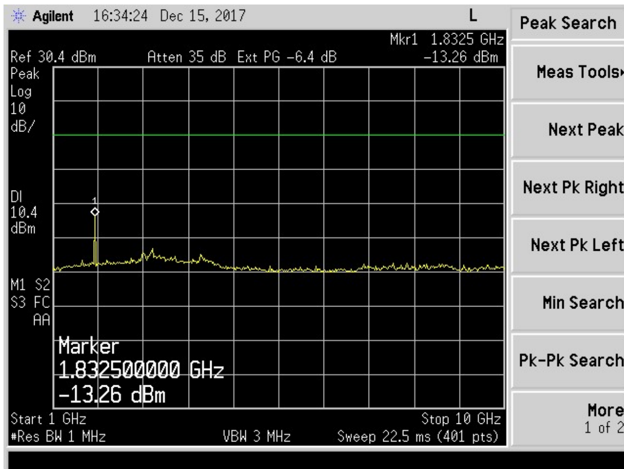
Figure 5. Antenna Conducted Emissions Low, 1 to 10 GHz
