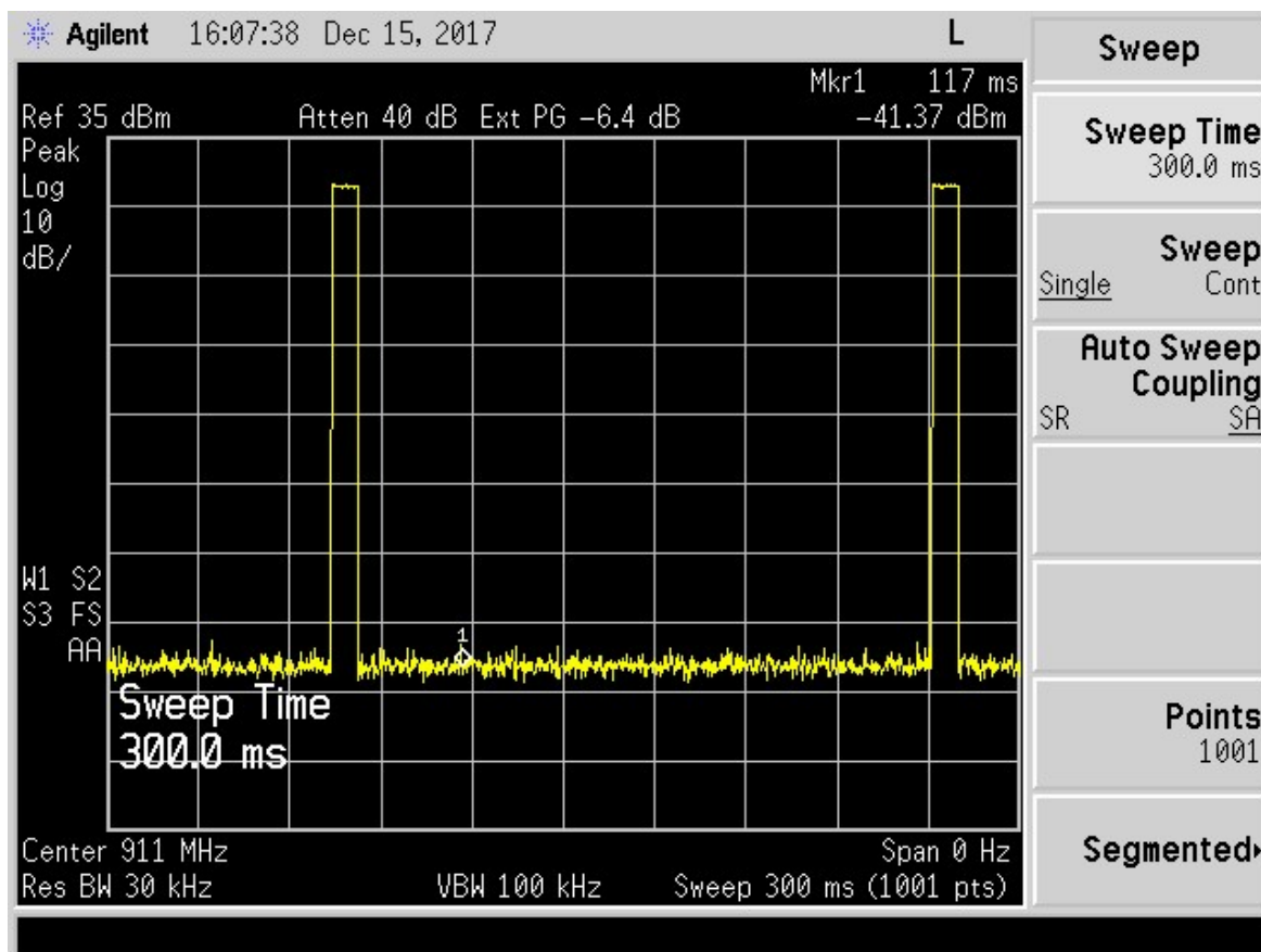
Figure 3. Pulse Train (Duty Cycle)
